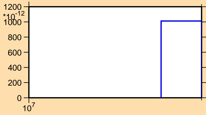
\sigma vs. E for ^{76}\text{Kr}(n,\text{nd})
