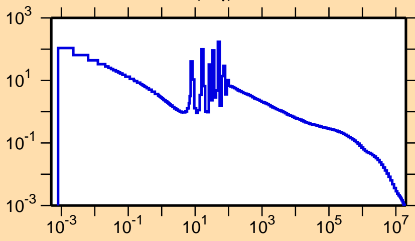
\sigma vs. E for ^{77}\text{Kr}(n,\gamma)
