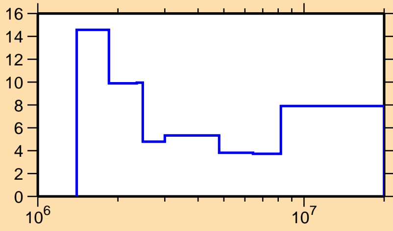
\Delta\sigma/\sigma vs. E for ^{77}\text{Kr}(n,tot.)
