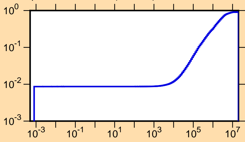
\mu vs. E for ^{78}\text{Kr}(\text{mt251})
