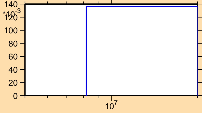
\sigma vs. E for ^{78}\text{Kr}(n,2n)
