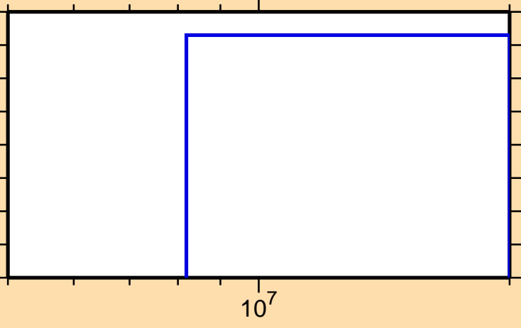
\sigma vs. E for ^{78}\text{Kr}(\text{mt } 45)
