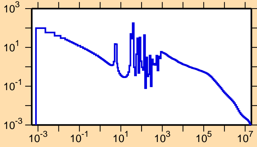
\sigma vs. E for ^{79}\text{Kr}(n,\gamma)
