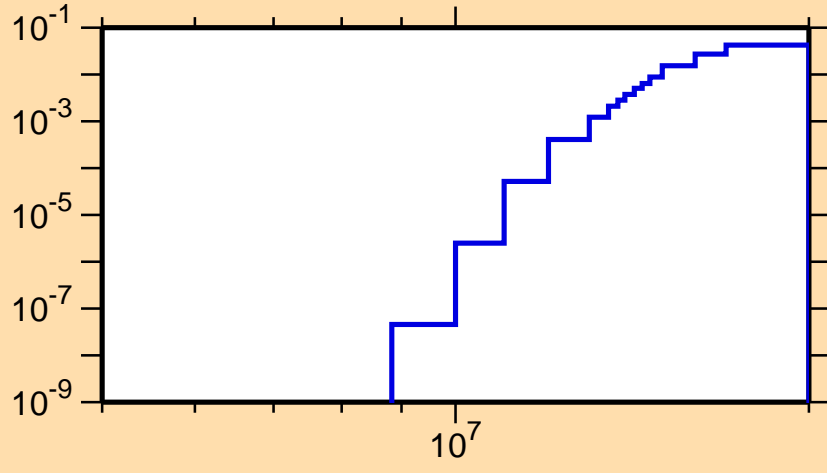
\sigma vs. E for ^{79}\text{Kr}(n, n\alpha)
