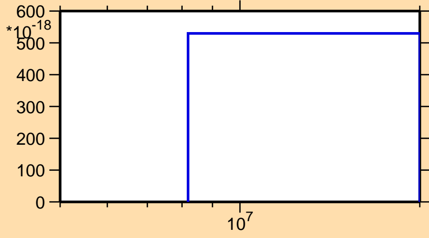
\sigma vs. E for ^{79}\text{Kr}(\text{mt117})
