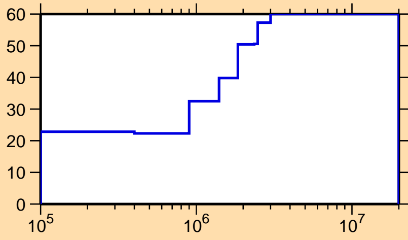
\Delta\sigma/\sigma vs. E for ^{79}\text{Kr}(n,n_1)
