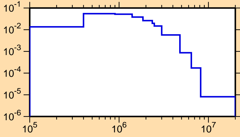
\sigma vs. E for ^{79}\text{Kr}(n,n_1)
