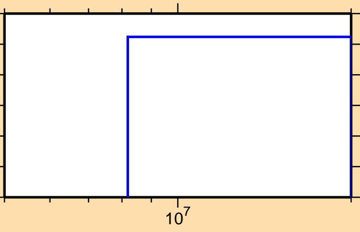
\sigma vs. E for ^{79}\text{Kr}(n,t)
