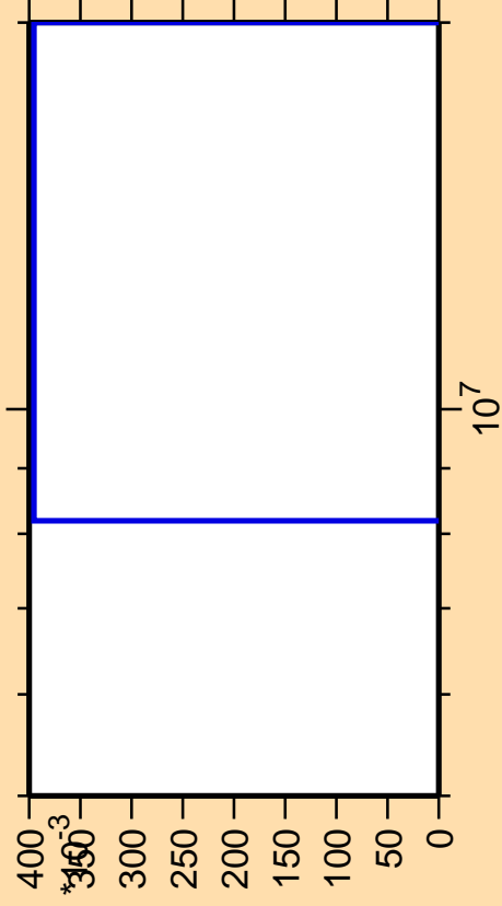
\Delta\sigma/\sigma vs. E for ^{79}\text{Kr}(\text{mt } 34)
