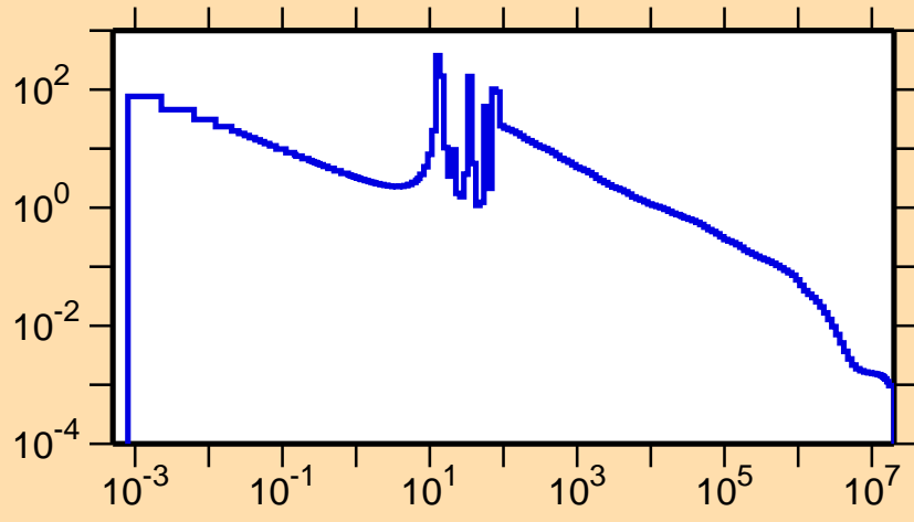
\sigma vs. E for ^{81}\text{Kr}(n,\gamma)
