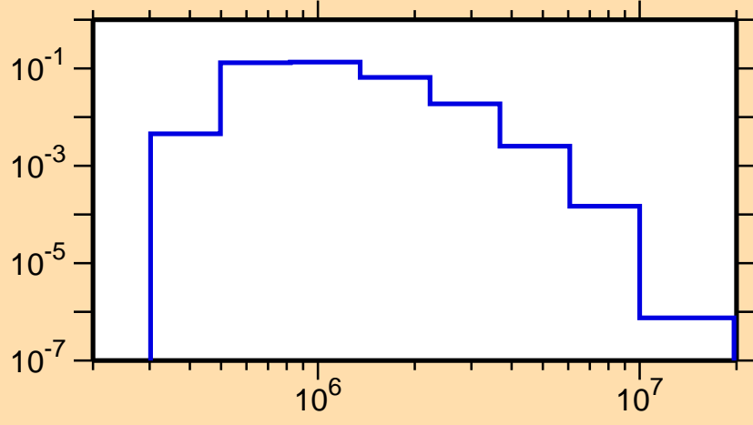
\sigma vs. E for ^{81}\text{Kr}(n,n_3)
