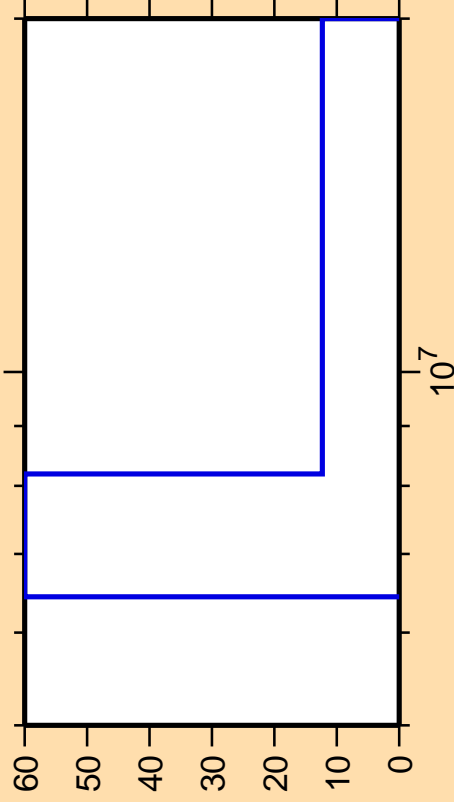
\Delta\sigma/\sigma vs. E for ^{81}\text{Kr}(n,2n)
