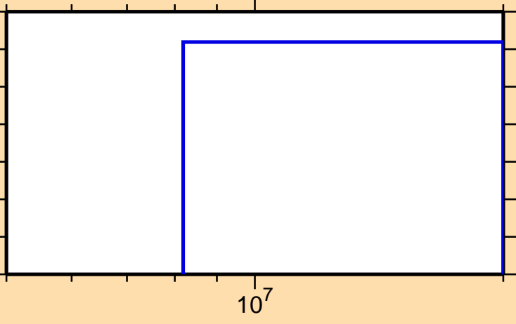
\sigma vs. E for ^{81}\text{Kr}(n,3n)
