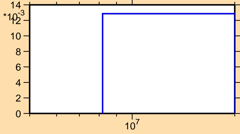
\sigma vs. E for ^{81}\text{Kr}(n,np)
