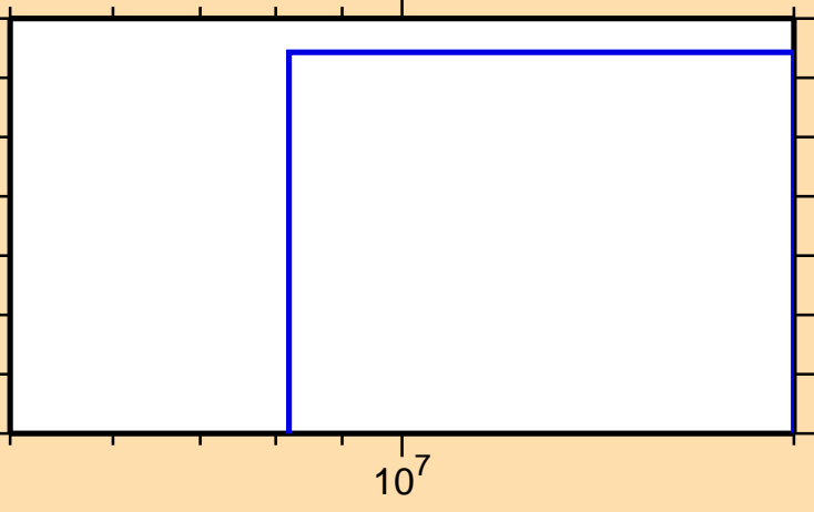
\sigma vs. E for ^{81}\text{Kr}(n,np)
