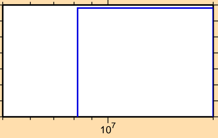
\sigma vs. E for ^{81}\text{Kr}(n,n\alpha)
