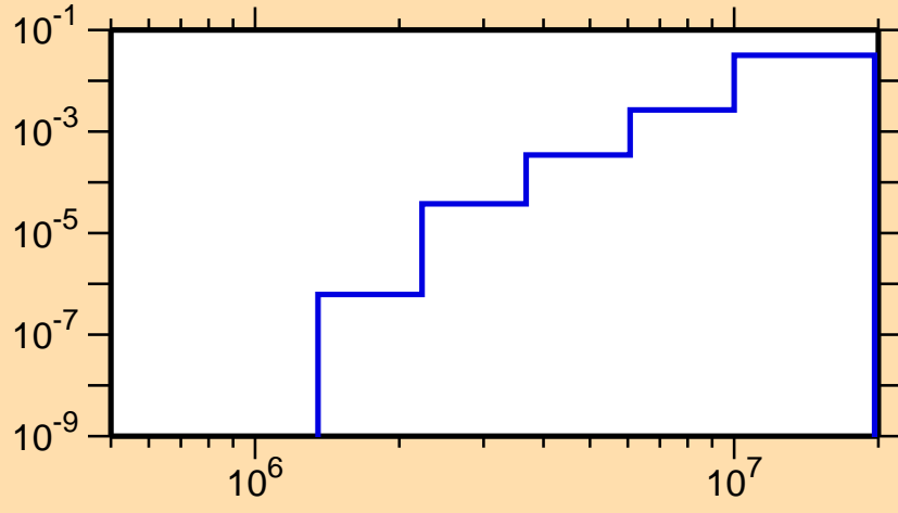
\sigma vs. E for ^{83}\text{Kr}(n,p)
