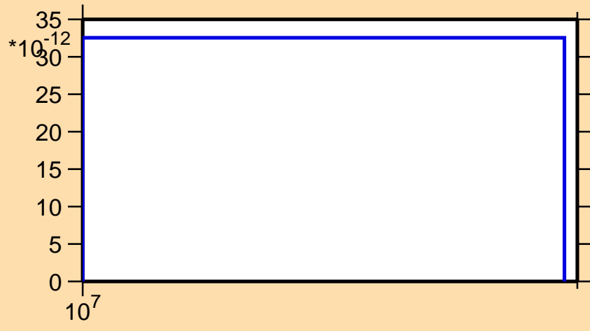
\sigma vs. E for ^{83}\text{Kr}(n,2np)
