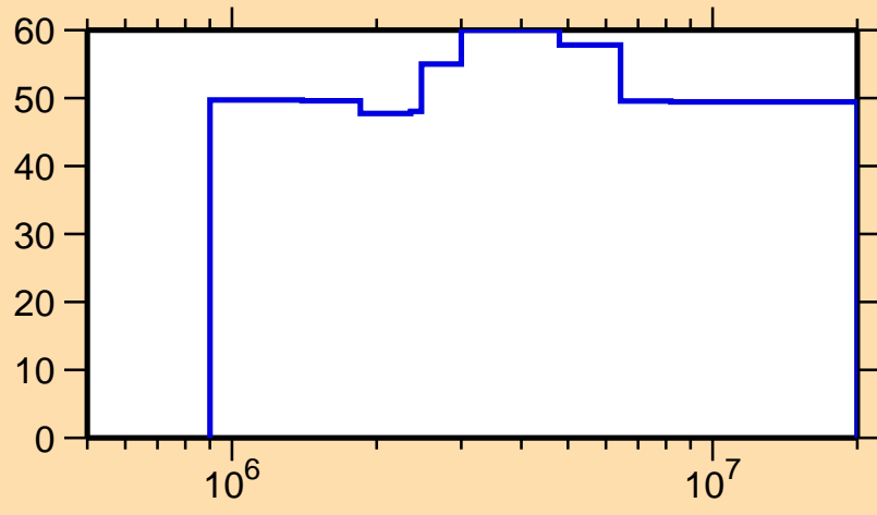
\Delta\sigma/\sigma vs. E for ^{83}\text{Kr}(n,p)
