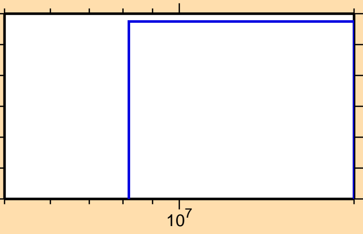
\sigma vs. E for ^{83}\text{Kr}(n,\text{He}3)
