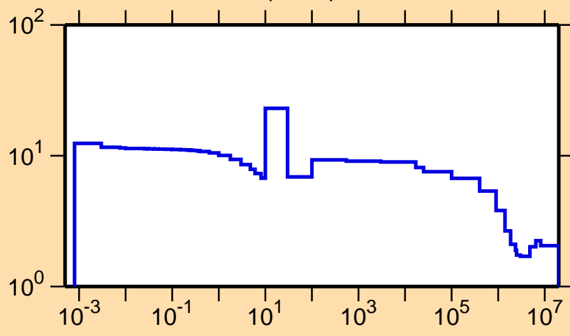
\sigma vs. E for ^{83}\text{Kr}(n,\text{el.})
