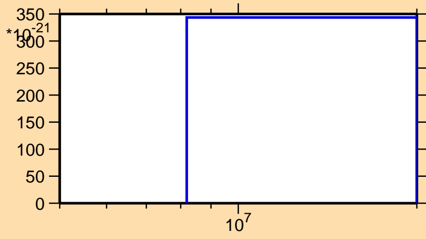
\sigma vs. E for ^{83}\text{Kr}(n,\text{pt})
