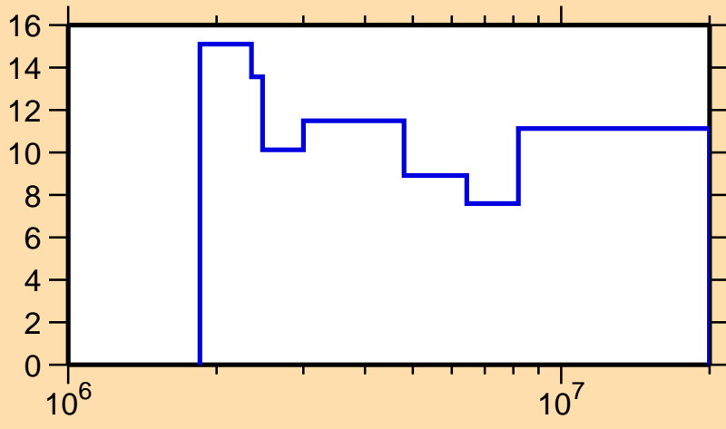
\Delta\sigma/\sigma vs. E for ^{83}\text{Kr}(n, el.)
