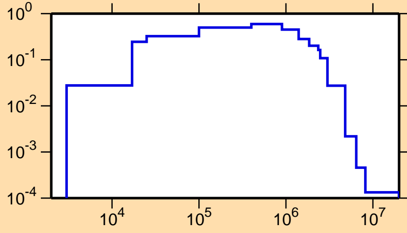
\sigma vs. E for ^{83}\text{Kr}(n,n_1)
