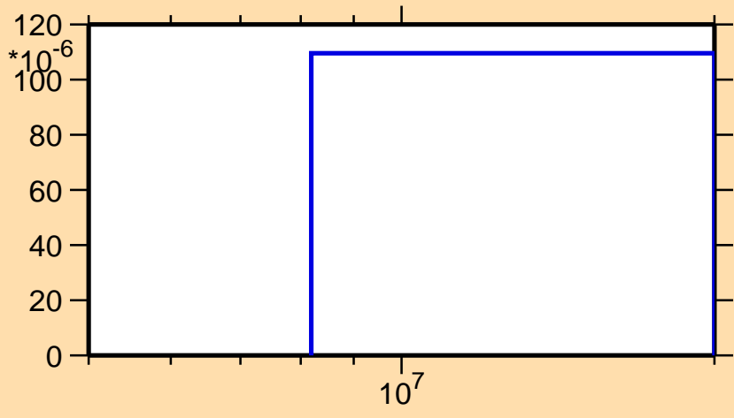
\sigma vs. E for ^{83}\text{Kr}(n,n\alpha)
