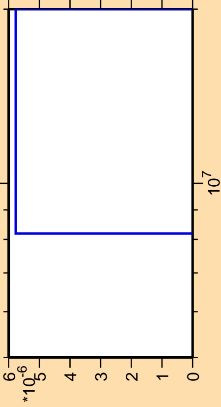
\Delta\sigma/\sigma vs. E for ^{83}\text{Kr}(n,\text{pt})
