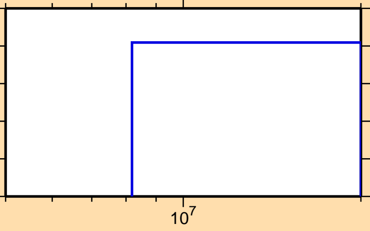
\sigma vs. E for ^{83}\text{Kr}(n,\text{pt})
