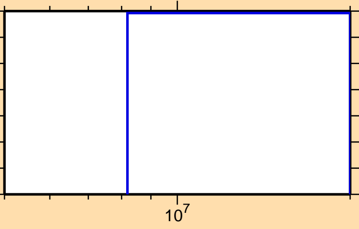
\sigma vs. E for ^{83}\text{Kr}(n,\text{nd})
