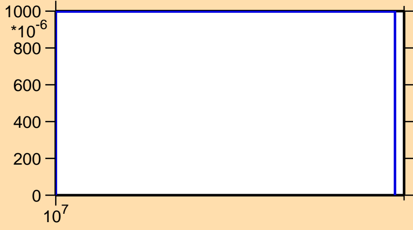
\sigma vs. E for ^{84}\text{Kr}(n,np)
