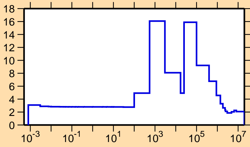
\sigma vs. E for ^{84}\text{Kr}(n,\text{el.})
