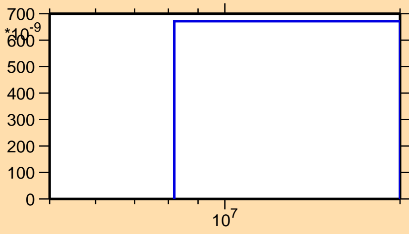
\sigma vs. E for ^{84}\text{Kr}(n,t)
