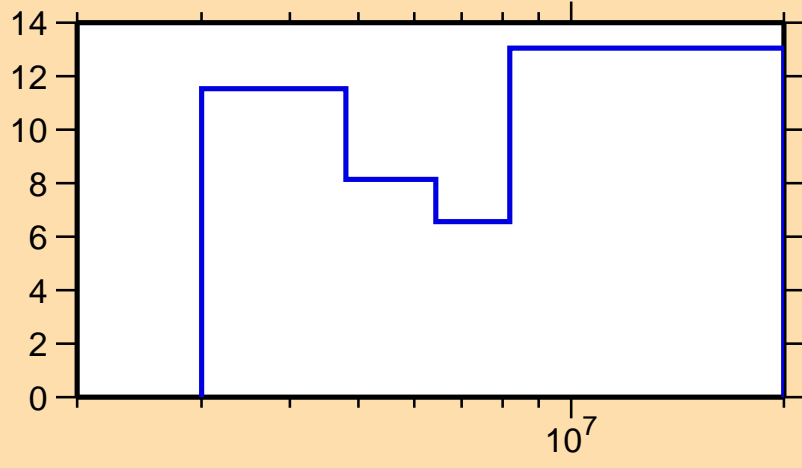
\Delta\sigma/\sigma vs. E for ^{84}\text{Kr}(n,el.)
