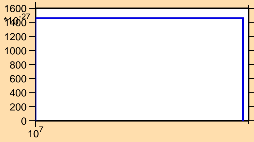
\sigma vs. E for ^{85}\text{Kr}(n,\text{pd})
