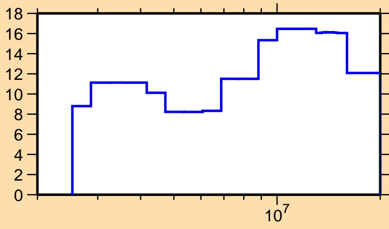
\Delta\sigma/\sigma vs. E for ^{87}\text{Kr}(n, el.)
