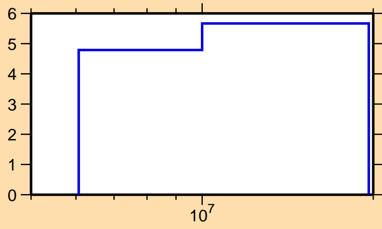
\Delta\sigma/\sigma vs. E for ^{87}\text{Kr}(n,\text{nonel.})
