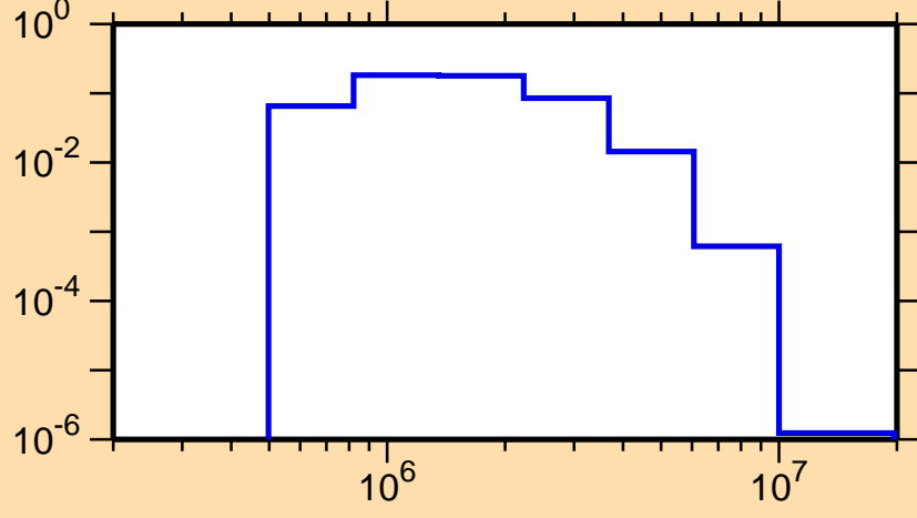
\sigma vs. E for ^{87}\text{Kr}(n,n_1)
