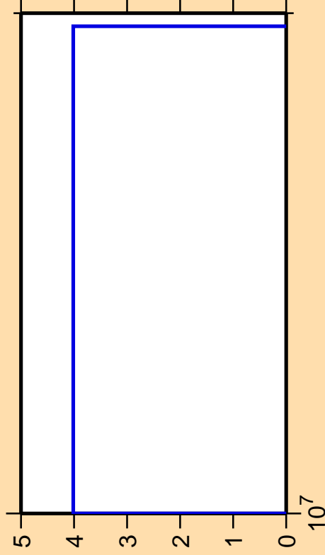
\Delta\sigma/\sigma vs. E for ^{87}\text{Kr}(n,2np)
