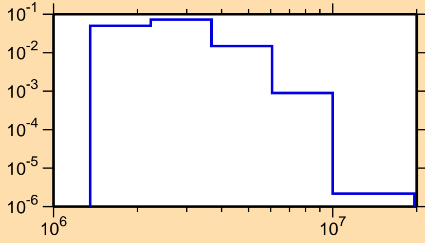
\sigma vs. E for ^{87}\text{Kr}(n,n_4)
