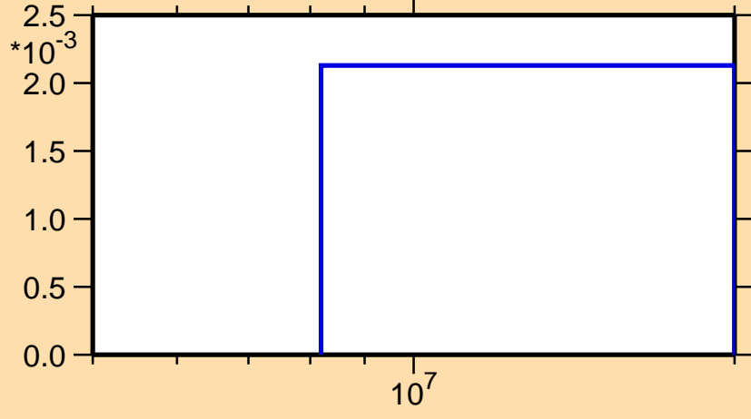
\sigma vs. E for ^{87}\text{Kr}(n,3n)
