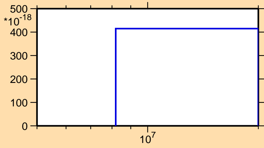
\sigma vs. E for ^{87}\text{Kr}(n,nt)
