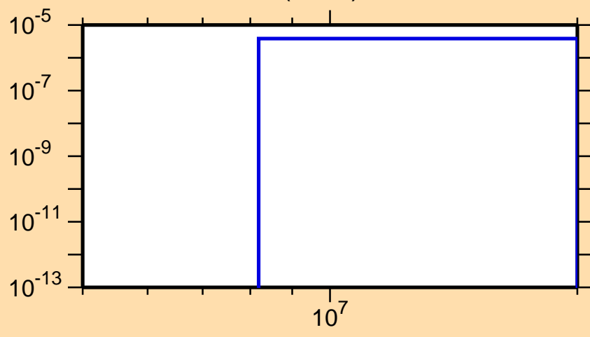
\sigma vs. E for ^{87}\text{Kr}(n,n\alpha)
