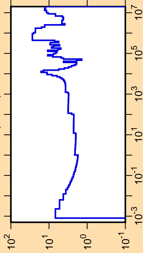
\Delta\sigma/\sigma vs. E for ^{88}\text{Kr}(n,\text{tot.})
