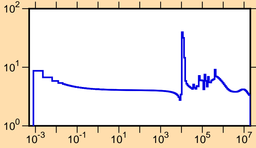
\sigma vs. E for ^{88}\text{Kr}(n,\text{tot.})
