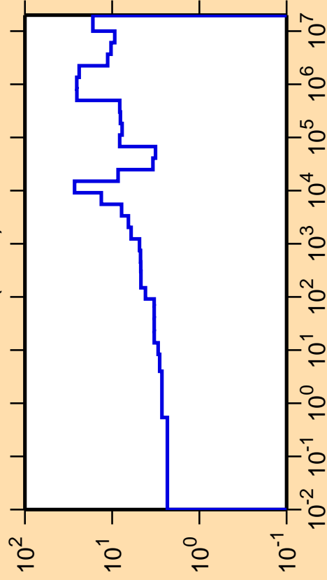
\Delta\sigma/\sigma vs. E for ^{88}\text{Kr}(n,\text{el.})
