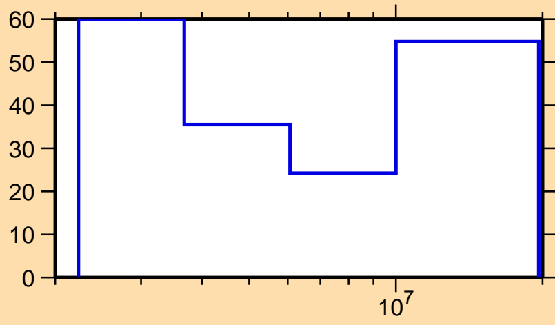
\Delta\sigma/\sigma vs. E for ^{88}\text{Kr}(n,n\text{cont.})
