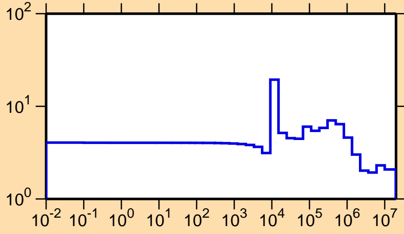
\sigma vs. E for ^{88}\text{Kr}(n,\text{el.})
