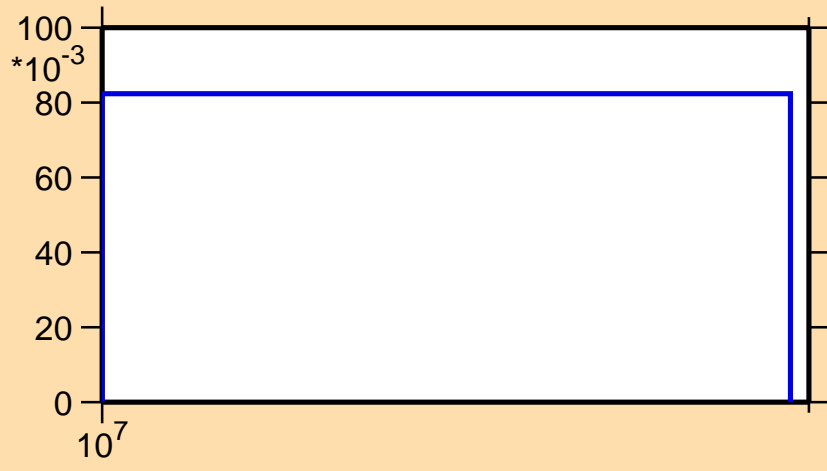
\sigma vs. E for ^{88}\text{Kr}(n,3n)
