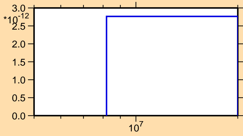
\sigma vs. E for ^{88}\text{Kr}(n,nd)
