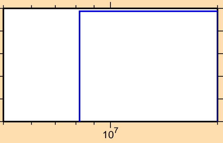
\sigma vs. E for ^{88}\text{Kr}(n,\alpha)
