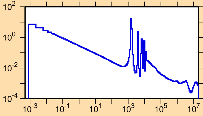
\sigma vs. E for ^{89}\text{Kr}(n,\gamma)
