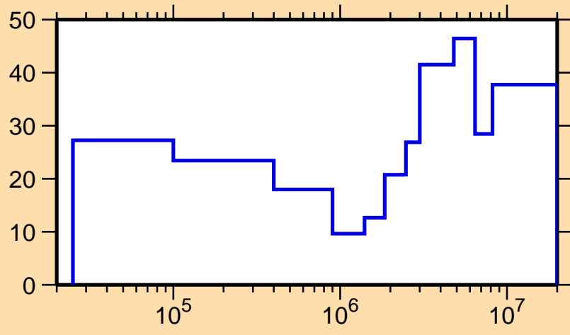
\Delta\sigma/\sigma vs. E for ^{89}\text{Kr}(n,n_1)
