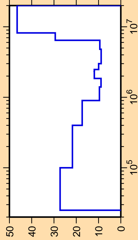
\Delta\sigma/\sigma vs. E for ^{89}\text{Kr}(n,\text{inel.})
