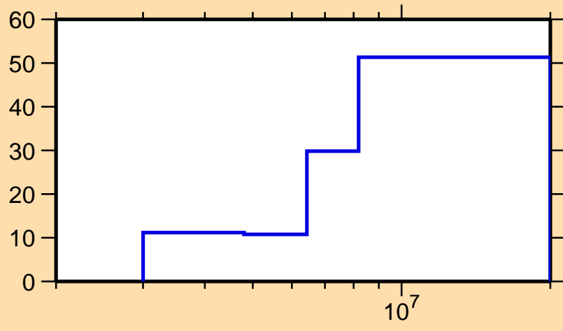
\Delta\sigma/\sigma vs. E for ^{89}\text{Kr}(n,n\text{cont.})
