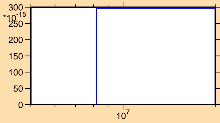
\sigma vs. E for ^{89}\text{Kr}(n,2np)
