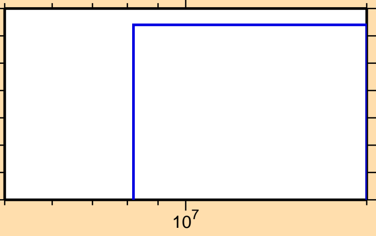
\sigma vs. E for ^{89}\text{Kr}(n,\text{nd})
