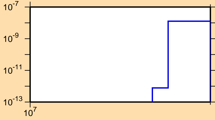
\sigma vs. E for ^{90}\text{Kr}(n,nt)
