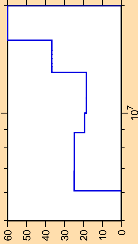
\Delta\sigma/\sigma vs. E for ^{90}\text{Kr}(n,2n)
