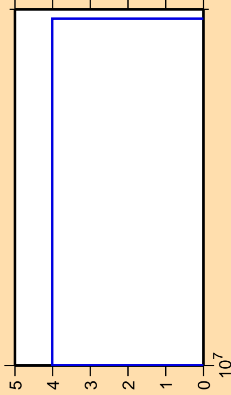
\Delta\sigma/\sigma vs. E for ^{90}\text{Kr}(n,nd)
