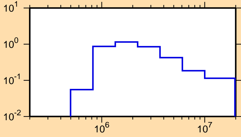
\sigma vs. E for ^{90}\text{Kr}(n,n_1)
