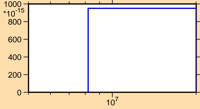
\sigma vs. E for ^{90}\text{Kr}(n,nd)
