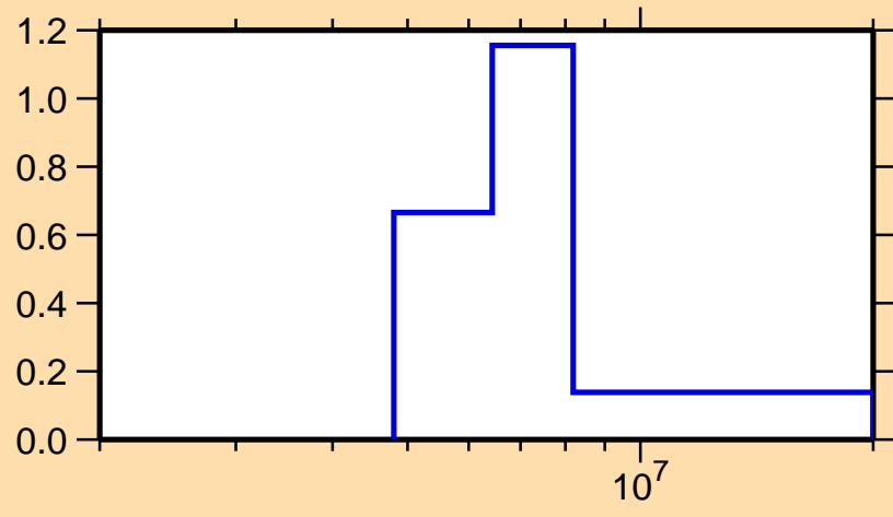
\sigma vs. E for ^{90}\text{Kr}(n,n\text{cont.})
