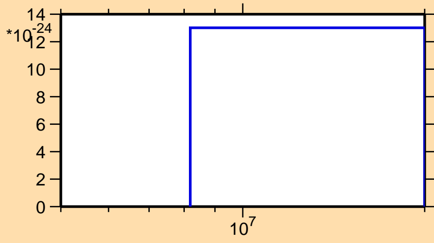
\sigma vs. E for ^{90}\text{Kr}(n,2np)
