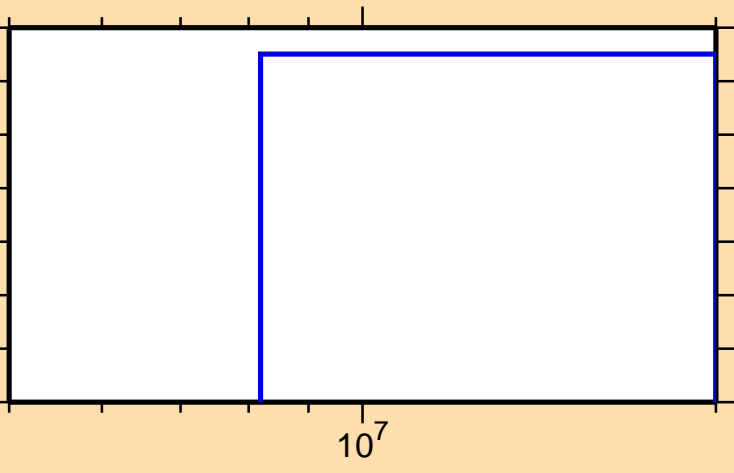
\sigma vs. E for ^{90}\text{Kr}(n,2np)
