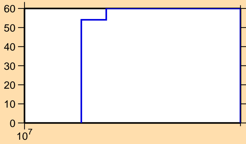
\Delta\sigma/\sigma vs. E for ^{92}\text{Kr}(n,el.)
