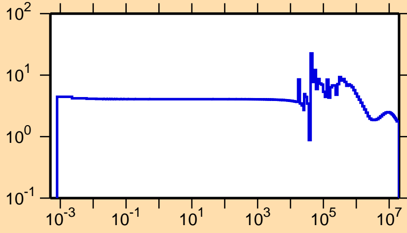
\sigma vs. E for ^{92}\text{Kr}(n,\text{el.})
