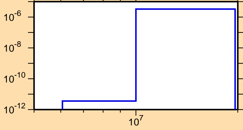
\sigma vs. E for ^{92}\text{Kr}(n,\alpha)
