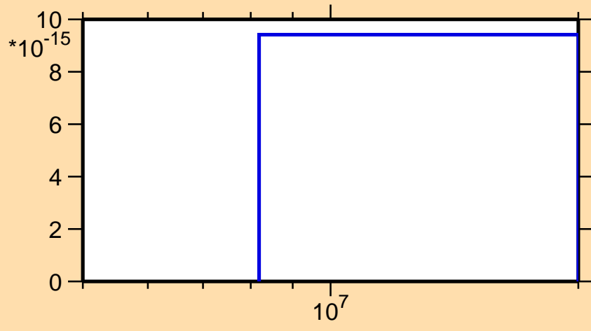
\sigma vs. E for ^{92}\text{Kr}(n,nd)
