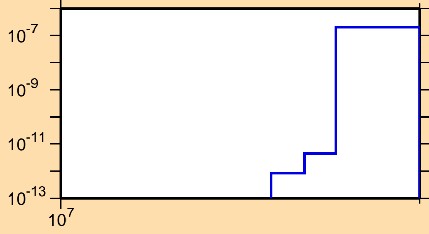
\sigma vs. E for ^{93}\text{Kr}(n,nt)
