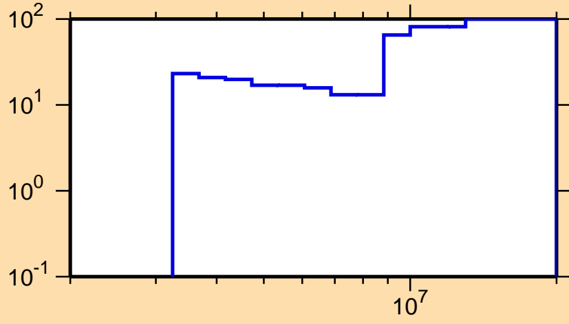
\Delta\sigma/\sigma vs. E for ^{93}\text{Kr}(n,2n)
