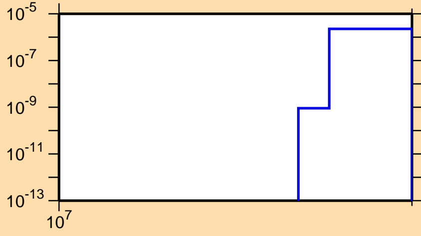
\sigma vs. E for ^{93}\text{Kr}(n,np)
