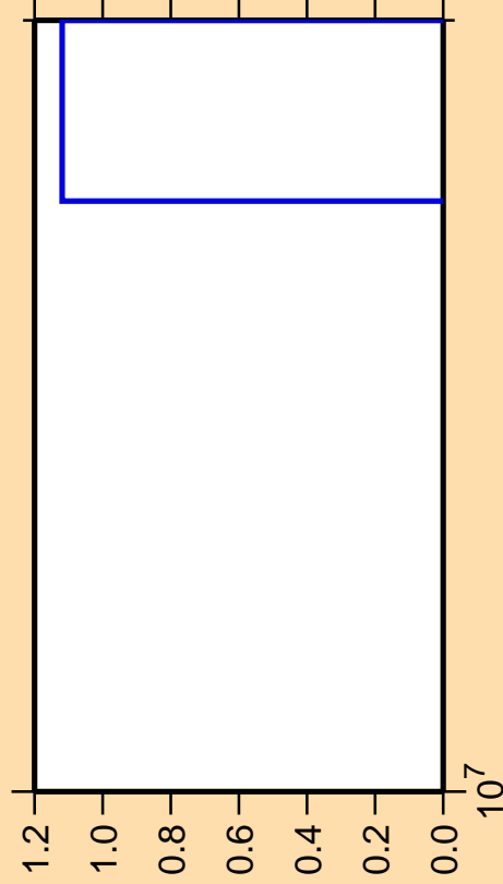
\Delta\sigma/\sigma vs. E for ^{93}\text{Kr}(n,2np)
