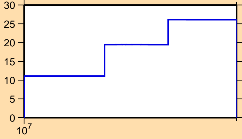
\Delta\sigma/\sigma vs. E for ^{93}\text{Kr}(n,el.)
