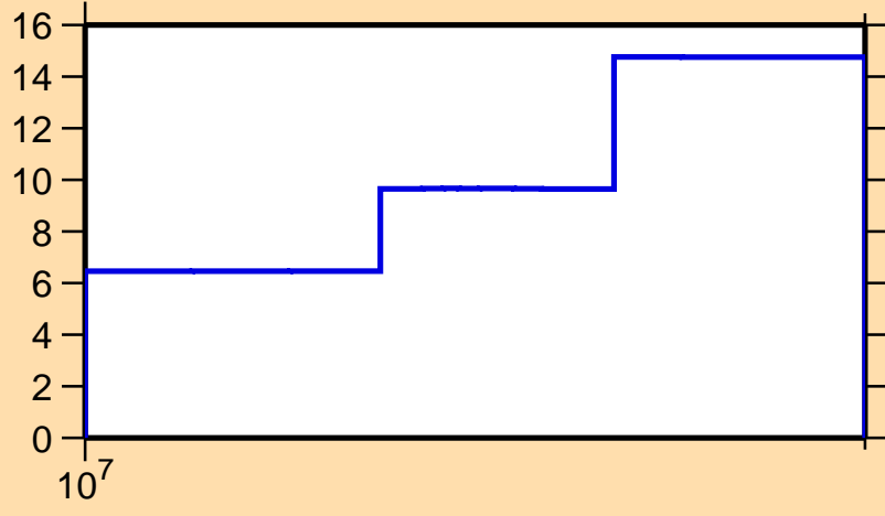
\Delta\sigma/\sigma vs. E for ^{93}\text{Kr}(n,\text{tot.})
