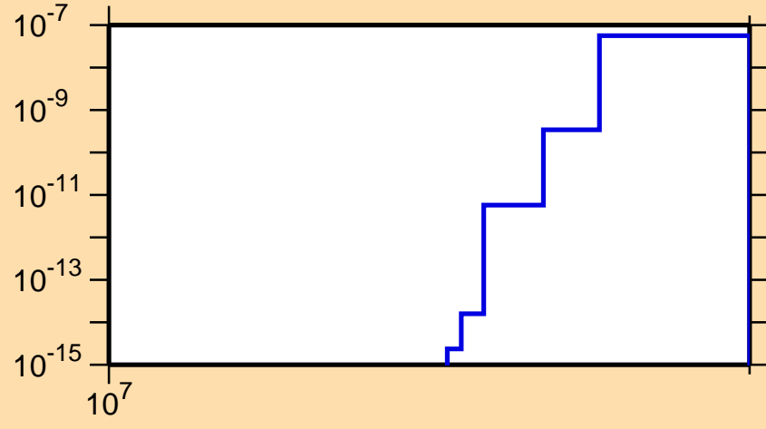
\sigma vs. E for ^{93}\text{Kr}(n,2n\alpha)
