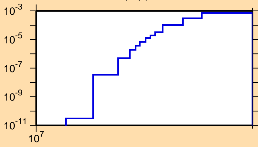
\sigma vs. E for ^{93}\text{Kr}(n,p)
