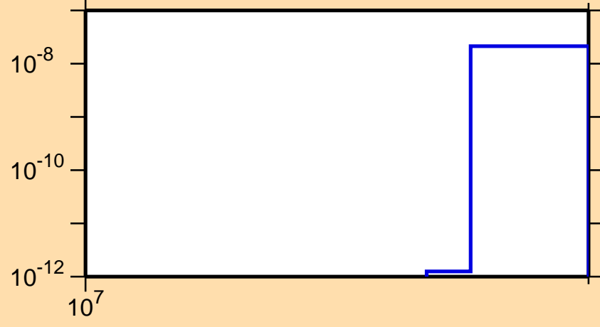
\sigma vs. E for ^{93}\text{Kr}(n,\text{nd})
