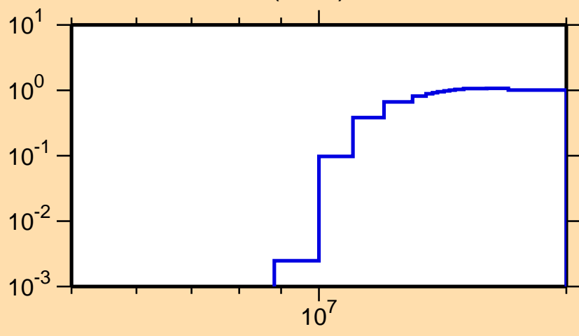
\sigma vs. E for ^{93}\text{Kr}(n,3n)
