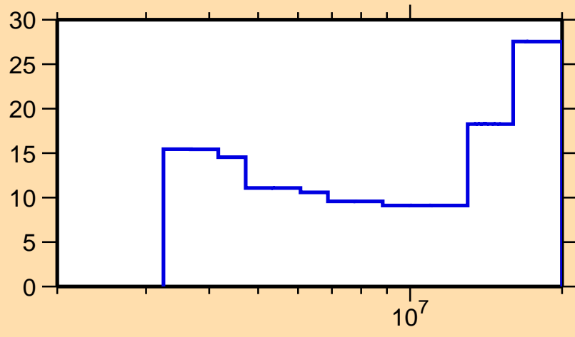
\Delta\sigma/\sigma vs. E for ^{93}\text{Kr}(n,\text{nonel.})
