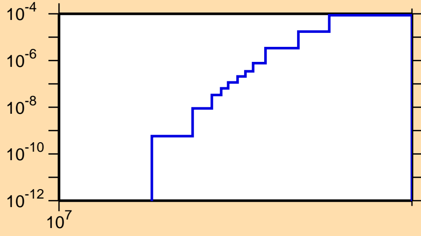
\sigma vs. E for ^{93}\text{Kr}(n,t)
