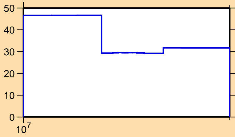
\Delta\sigma/\sigma vs. E for ^{93}\text{Kr}(n,\text{inel.})
