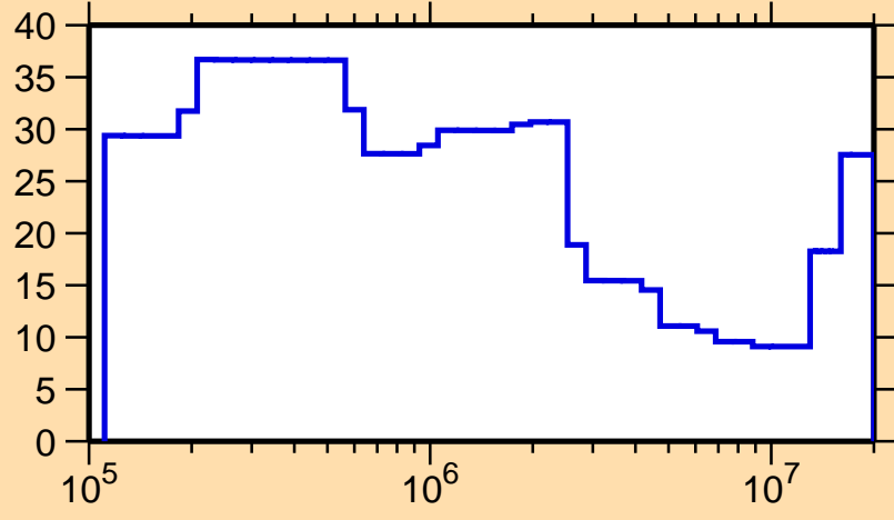
\Delta\sigma/\sigma vs. E for ^{93}\text{Kr}(n,\text{nonel.})
