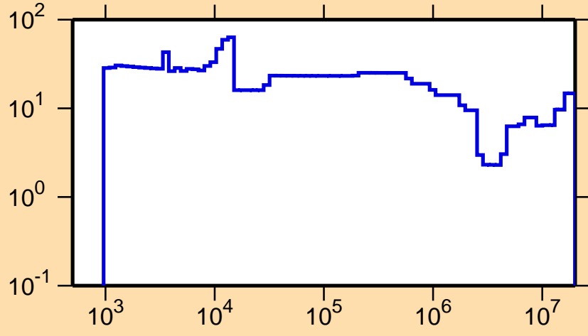
\Delta\sigma/\sigma vs. E for ^{93}\text{Kr}(n,\text{tot.})
