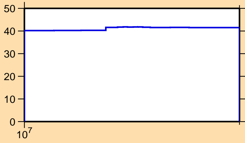
\Delta\sigma/\sigma vs. E for ^{93}\text{Kr}(n,n_1)
