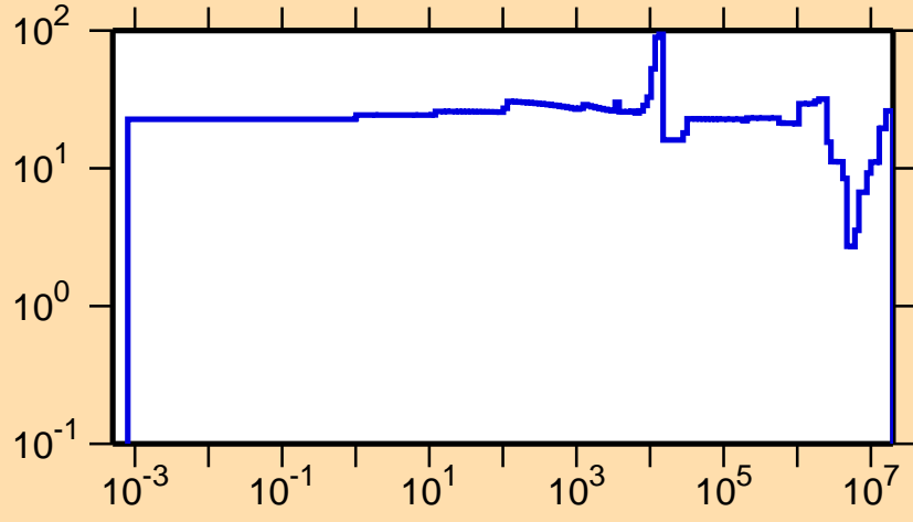
\Delta\sigma/\sigma vs. E for ^{93}\text{Kr}(n,\text{el.})
