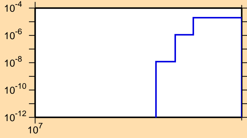
\sigma vs. E for ^{93}\text{Kr}(n,d)
