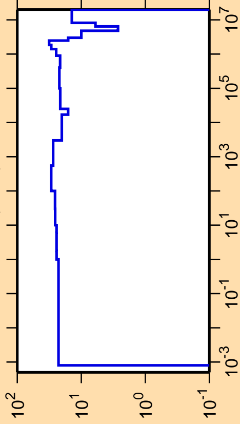
\Delta\sigma/\sigma vs. E for ^{93}\text{Kr}(n,\text{el.})
