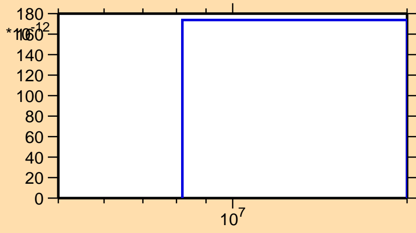
\sigma vs. E for ^{93}\text{Kr}(n,nd)
