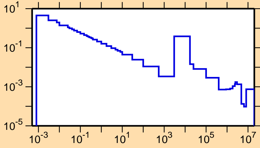
\sigma vs. E for ^{93}\text{Kr}(n,\gamma)
