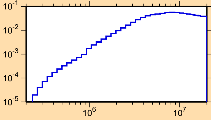
\sigma vs. E for ^{120}\text{La}(n,\text{inel.})
