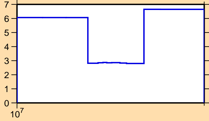
\Delta\sigma/\sigma vs. E for ^{120}\text{La}(n,\text{el.})
