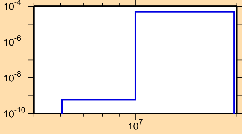
\sigma vs. E for ^{120}\text{La} (mt 45)
