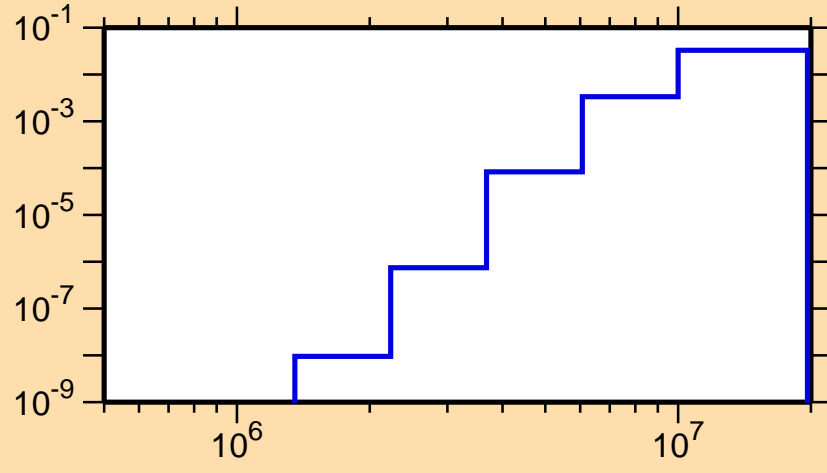
\sigma vs. E for ^{120}\text{La}(n,d)
