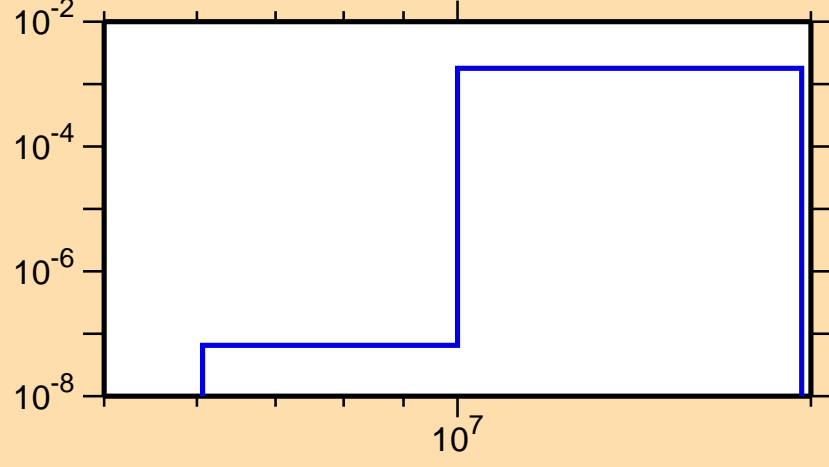
\sigma vs. E for ^{120}\text{La}(n,pd)
