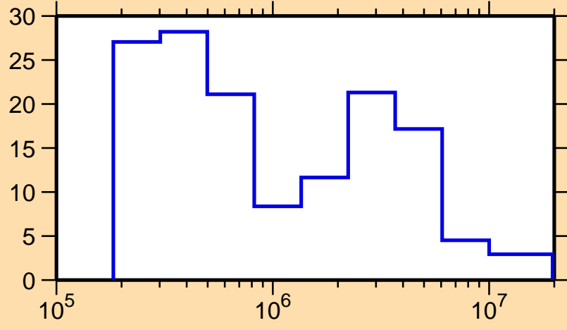
\Delta\sigma/\sigma vs. E for ^{120}\text{La}(n, el.)
