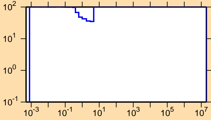
\Delta\sigma/\sigma vs. E for ^{120}\text{La}(n,\gamma)
