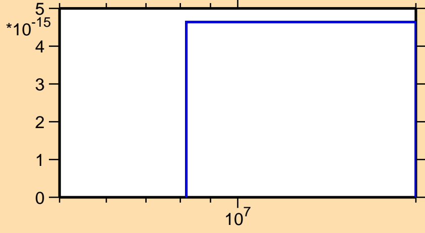
\sigma vs. E for ^{120}\text{La}(n,nt)
