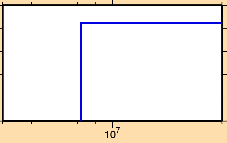
\sigma vs. E for ^{120}\text{La}(n,2n\alpha)
