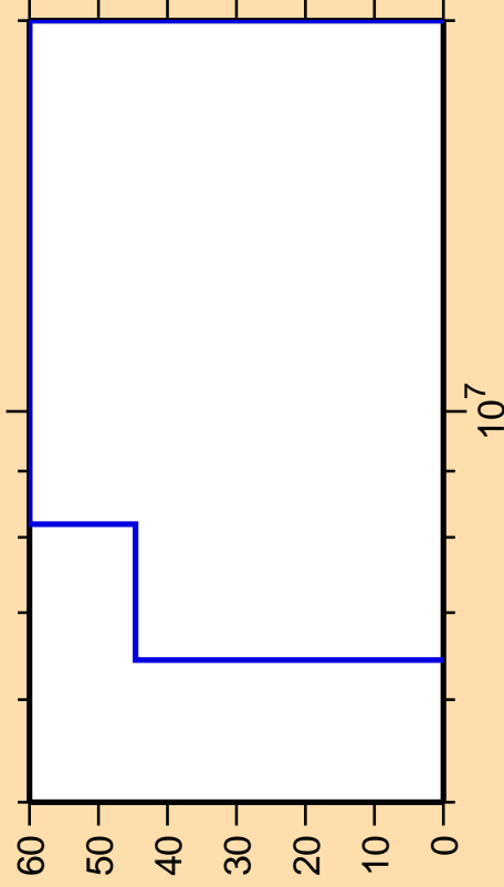
\Delta\sigma/\sigma vs. E for ^{120}\text{La}(\text{mt117})
