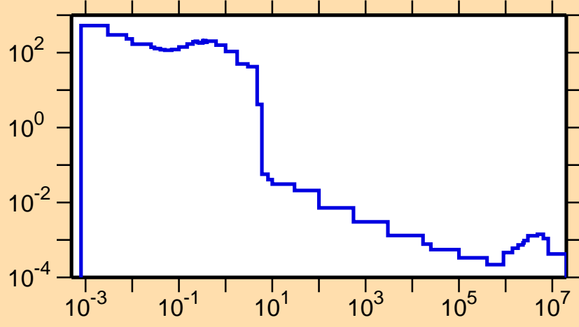
\sigma vs. E for ^{120}\text{La}(n,\gamma)
