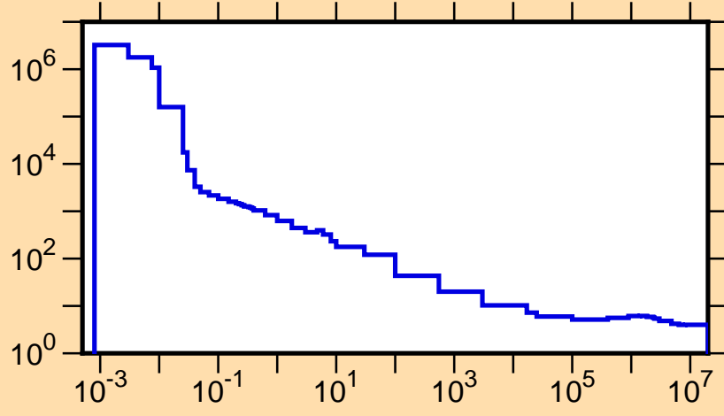
\sigma vs. E for ^{120}\text{La}(n,\text{tot.})
