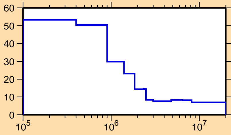
\Delta\sigma/\sigma vs. E for ^{120}\text{La}(n,\text{nonel.})
