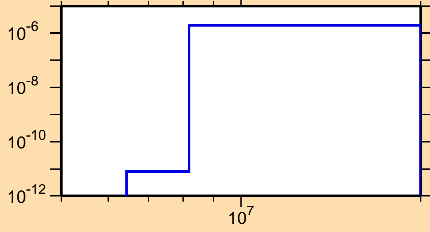
\sigma vs. E for ^{120}\text{La}(\text{mt117})
