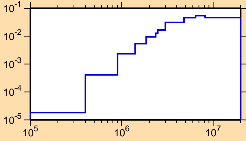
\sigma vs. E for ^{120}\text{La}(n,n\text{cont.})
