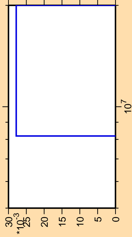
\Delta\sigma/\sigma vs. E for ^{120}\text{La}(n,nt)
