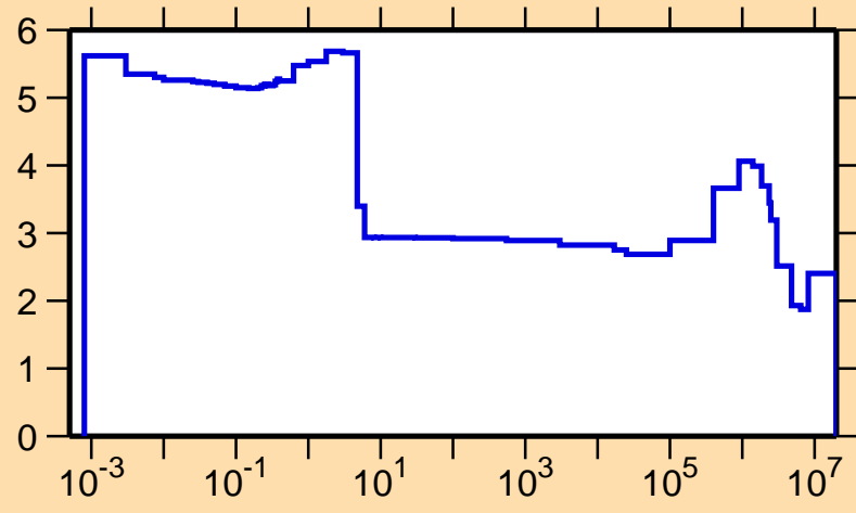
\sigma vs. E for ^{120}\text{La}(n,\text{el.})
