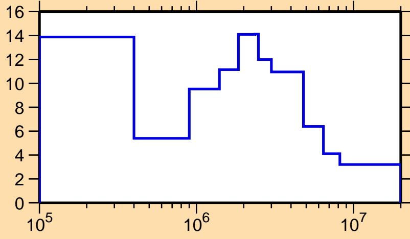
\Delta\sigma/\sigma vs. E for ^{120}\text{La}(n,\text{tot.})
