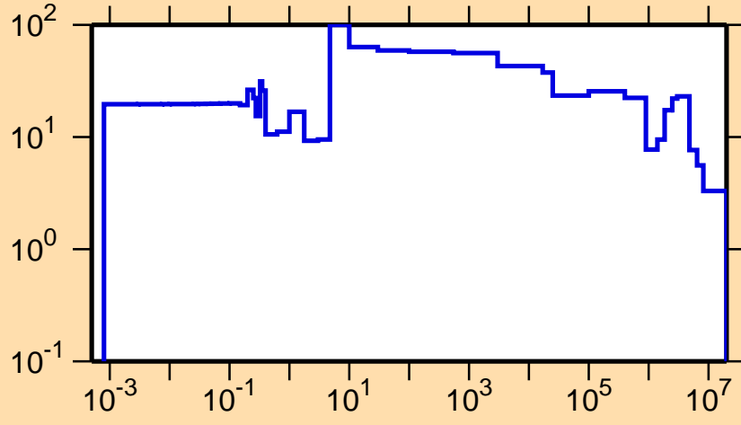
\Delta\sigma/\sigma vs. E for ^{120}\text{La}(n,\text{el.})
