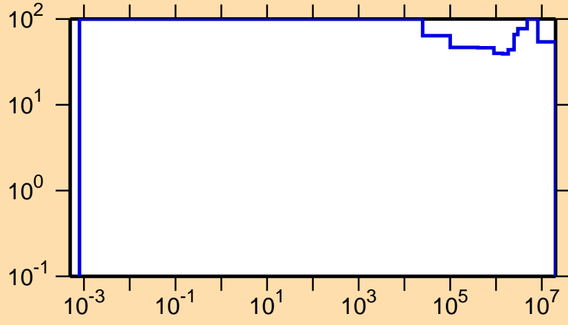
\Delta\sigma/\sigma vs. E for ^{120}\text{La}(n,p)
