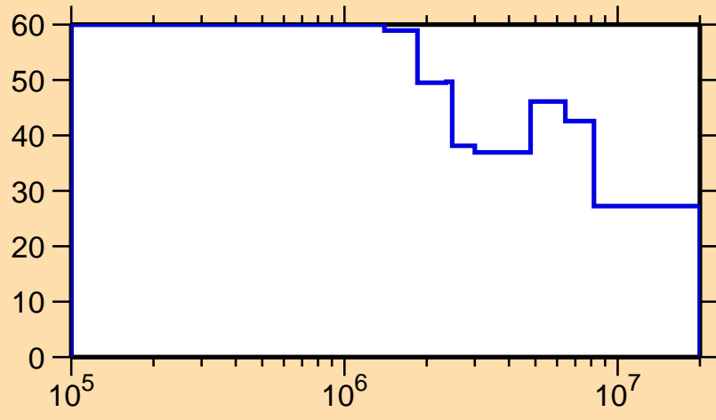
\Delta\sigma/\sigma vs. E for ^{120}\text{La}(n,n_1)
