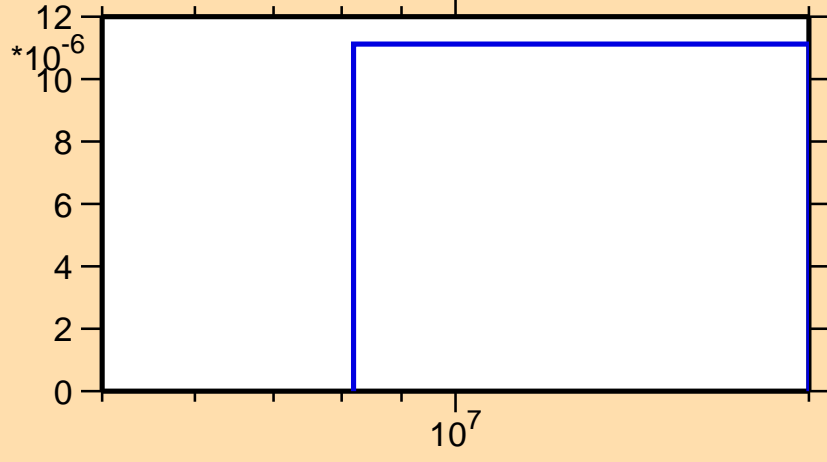
\sigma vs. E for ^{120}\text{La}(n,2np)
