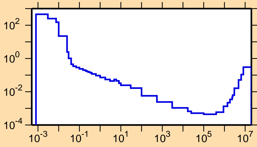
\sigma vs. E for ^{120}\text{La}(n,p\alpha)
