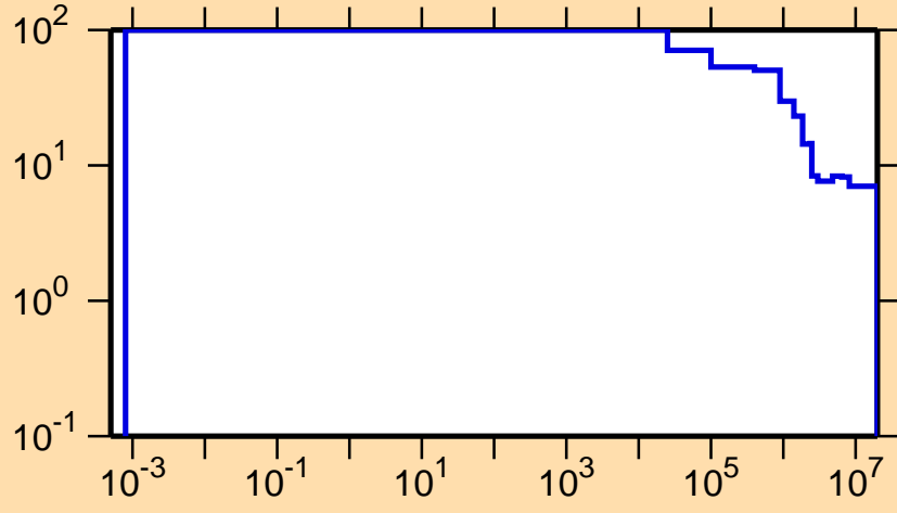
\Delta\sigma/\sigma vs. E for ^{120}\text{La}(n,\text{nonel.})
