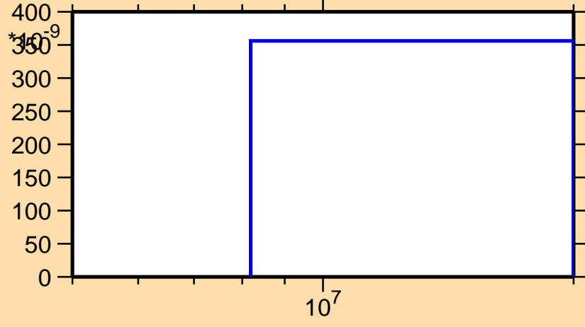
\sigma vs. E for ^{120}\text{La}(n,\text{nd})
