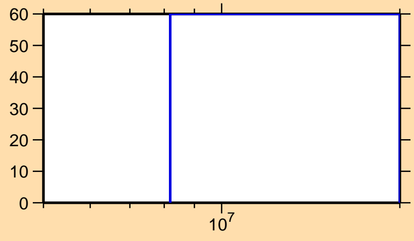
\Delta\sigma/\sigma vs. E for ^{120}\text{La}(n,2n)
