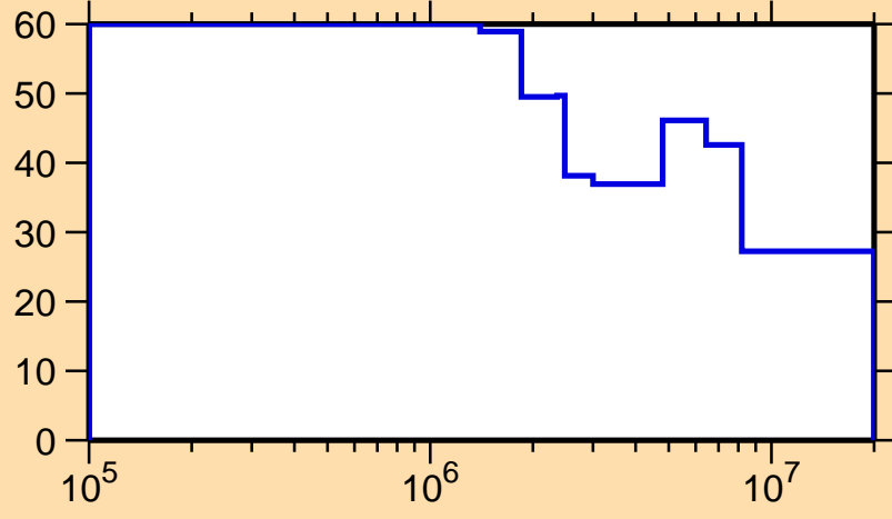
\Delta\sigma/\sigma vs. E for ^{120}\text{La}(n,n_1)
