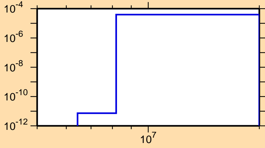
\sigma vs. E for ^{120}\text{La} (mt 45)
