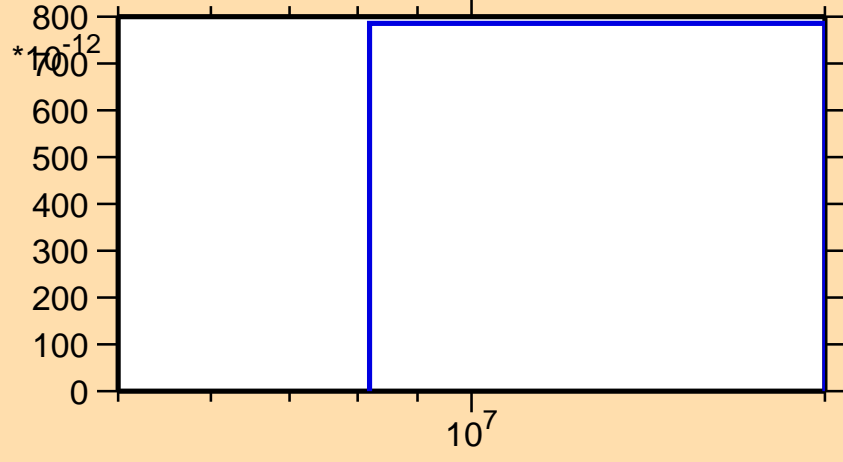
\sigma vs. E for ^{120}\text{La} (mt 34)
