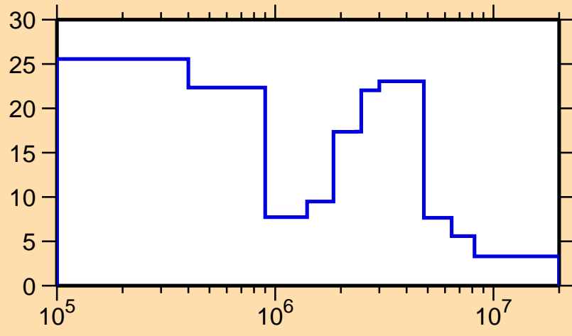
\Delta\sigma/\sigma vs. E for ^{120}\text{La}(n,\text{el.})
