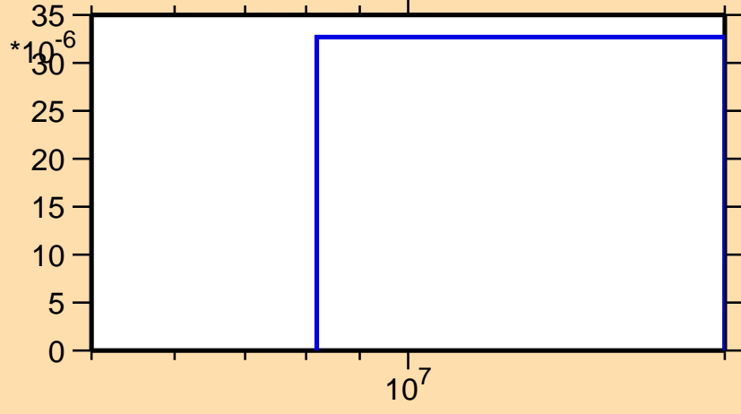
\sigma vs. E for ^{120}\text{La}(n,2n)
