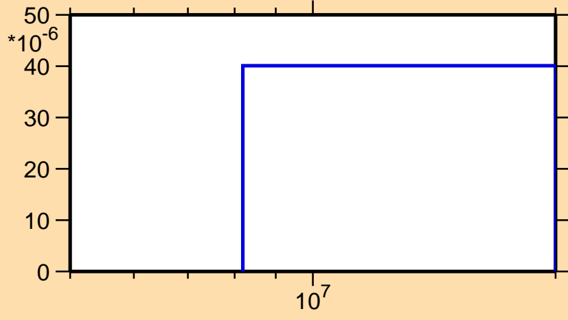
\sigma vs. E for ^{120}\text{La}(n,\text{pt})
