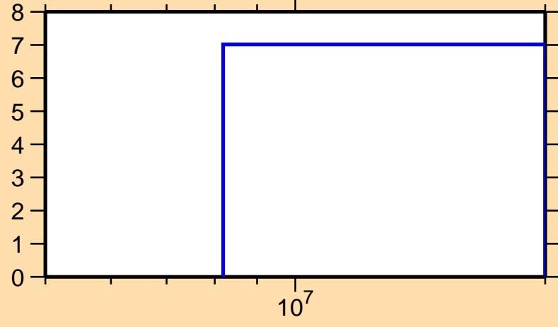
\Delta\sigma/\sigma vs. E for ^{120}\text{La}(n,\text{nonel.})
