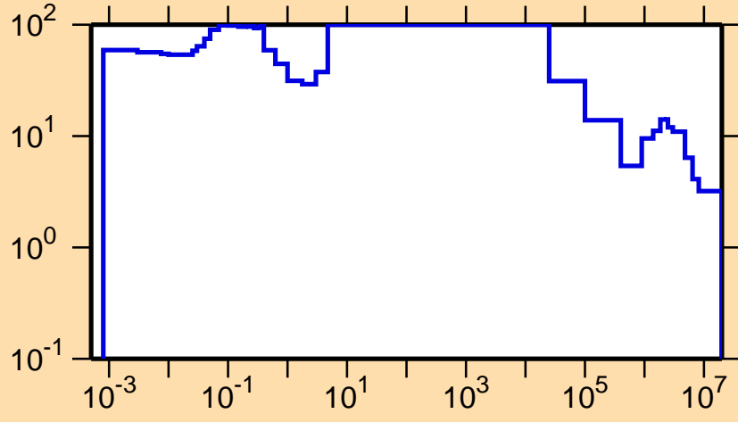
\Delta\sigma/\sigma vs. E for ^{120}\text{La}(n,\text{tot.})
