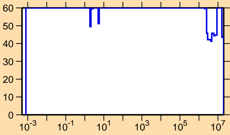
\Delta\sigma/\sigma vs. E for ^{121}\text{La}(n,\gamma)
