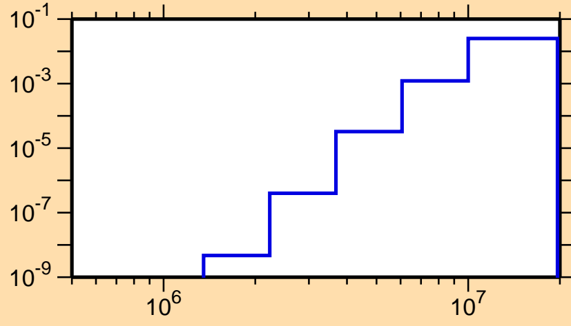
\sigma vs. E for ^{121}\text{La}(n,d)
