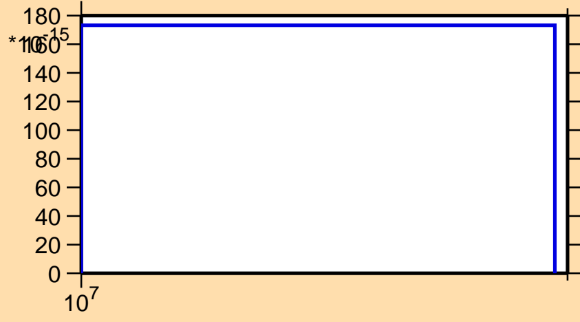
\sigma vs. E for ^{121}\text{La}(n,nt)
