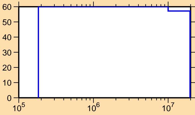
\Delta\sigma/\sigma vs. E for ^{121}\text{La}(n,n_1)
