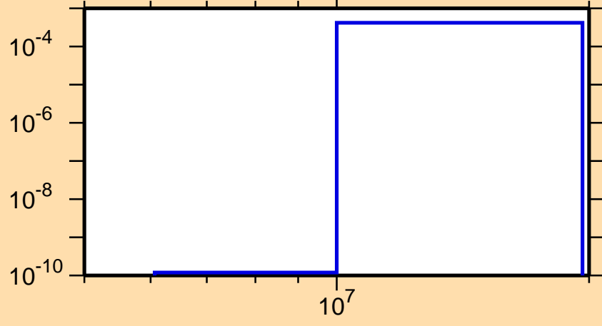
\sigma vs. E for ^{121}\text{La}(n,t)
