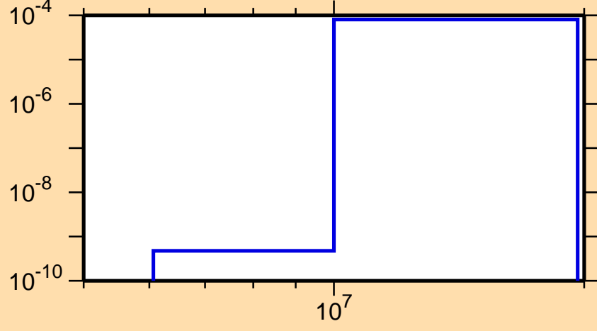
\sigma vs. E for ^{121}\text{La} (mt 45)
