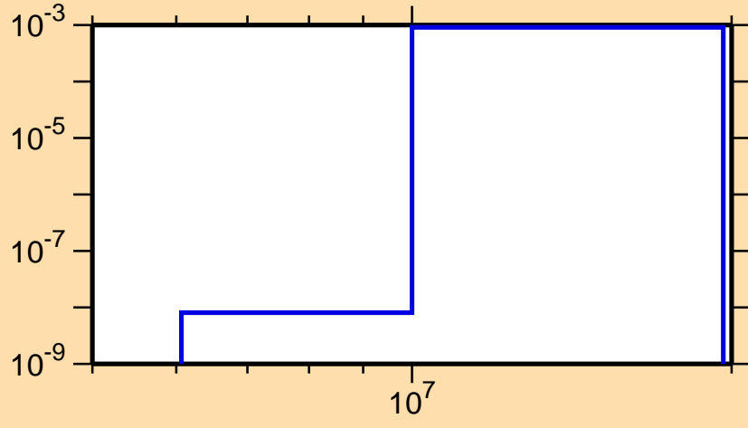
\sigma vs. E for ^{121}\text{La}(n,pd)
