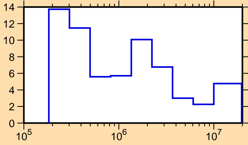
\Delta\sigma/\sigma vs. E for ^{121}\text{La}(n, \text{tot.})
