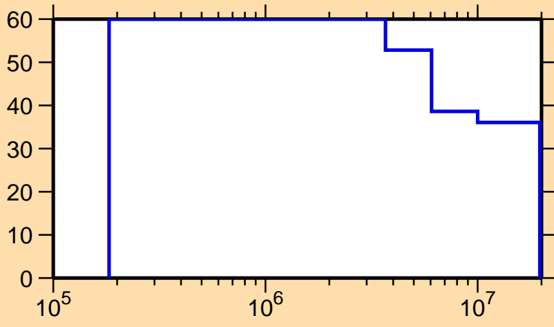
\Delta\sigma/\sigma vs. E for ^{121}\text{La}(n,n\text{cont.})
