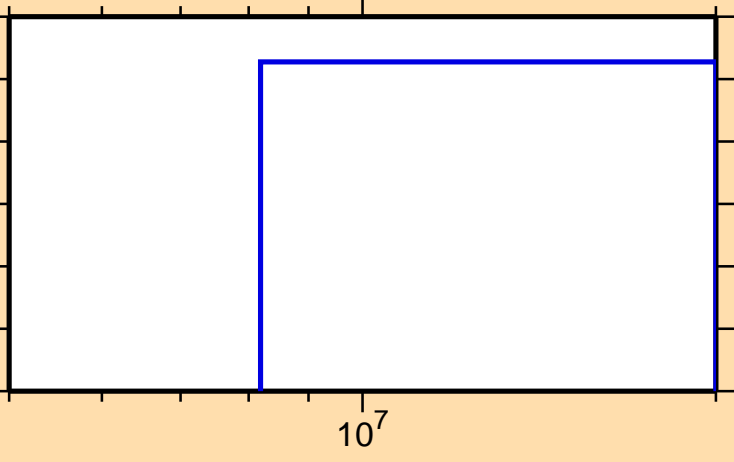
\sigma vs. E for ^{121}\text{La}(n,2n)
