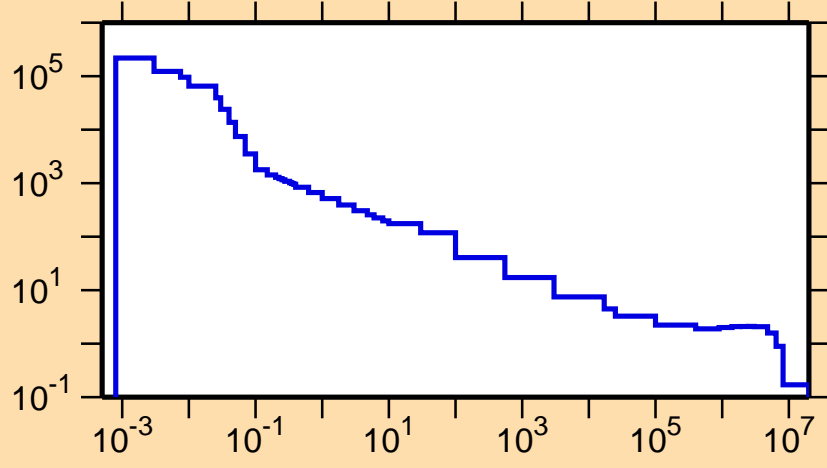
\sigma vs. E for ^{121}\text{La}(n,p)
