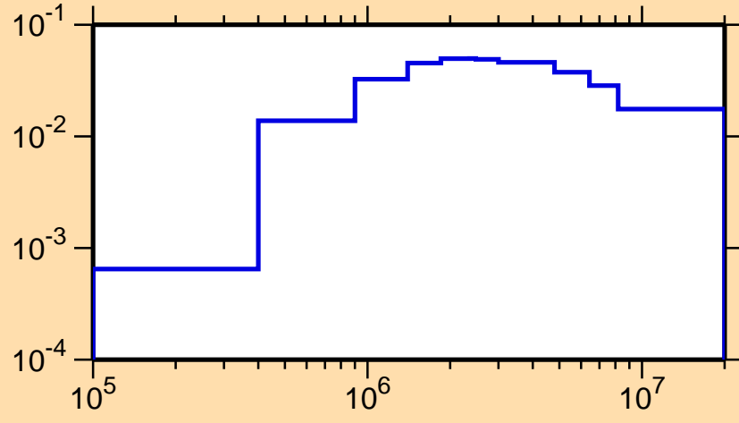
\sigma vs. E for ^{121}\text{La}(n,n_1)
