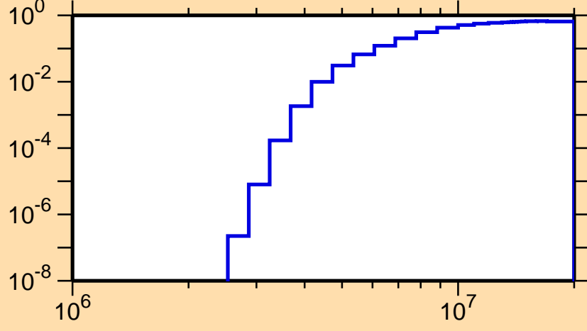
\sigma vs. E for ^{122}\text{La}(n,np)
