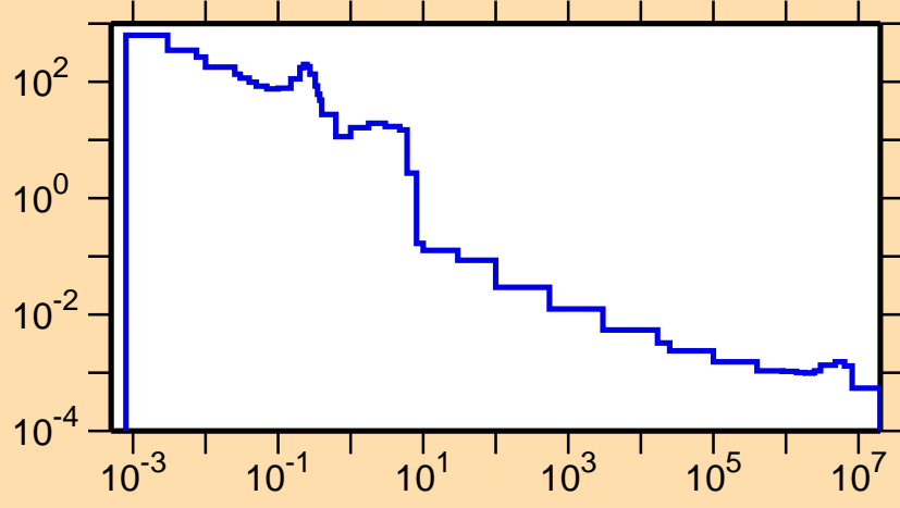
\sigma vs. E for ^{122}\text{La}(n,\gamma)
