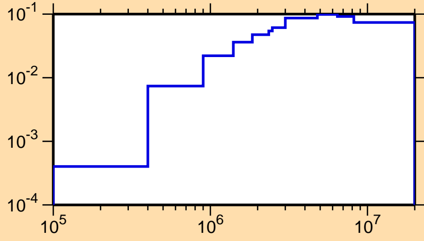
\sigma vs. E for ^{122}\text{La}(n,n\text{cont.})
