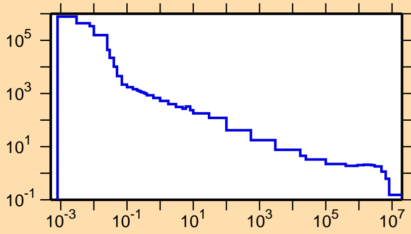
\sigma vs. E for ^{122}\text{La}(n,p)
