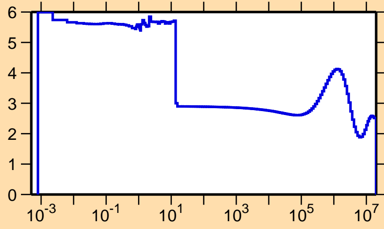
\sigma vs. E for ^{123}\text{La}(n,\text{el.})
