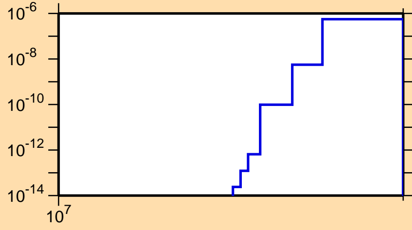
\sigma vs. E for ^{123}\text{La}(n,pt)
