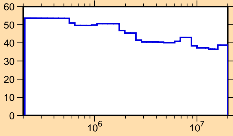
\Delta\sigma/\sigma vs. E for ^{123}\text{La}(n,n\text{onel.})
