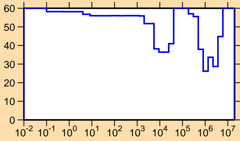
\Delta\sigma/\sigma vs. E for ^{124}\text{La}(n,p)
