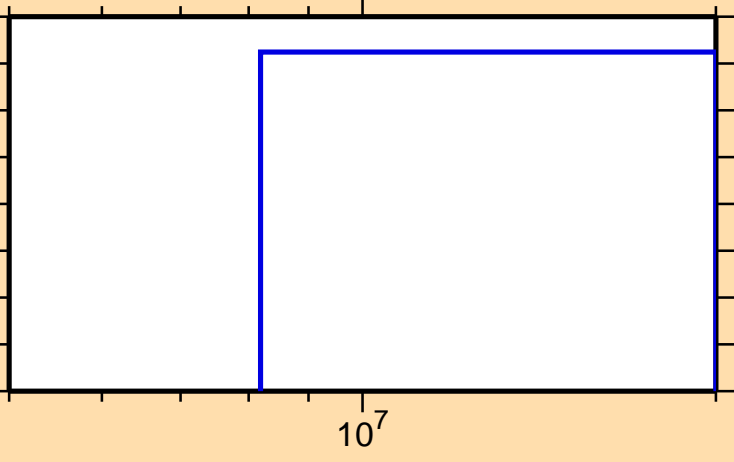
\sigma vs. E for ^{124}\text{La}(n,\text{nd})
