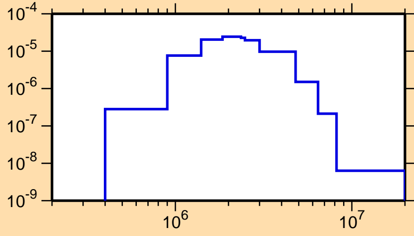
\sigma vs. E for ^{124}\text{La}(n,n_1)
