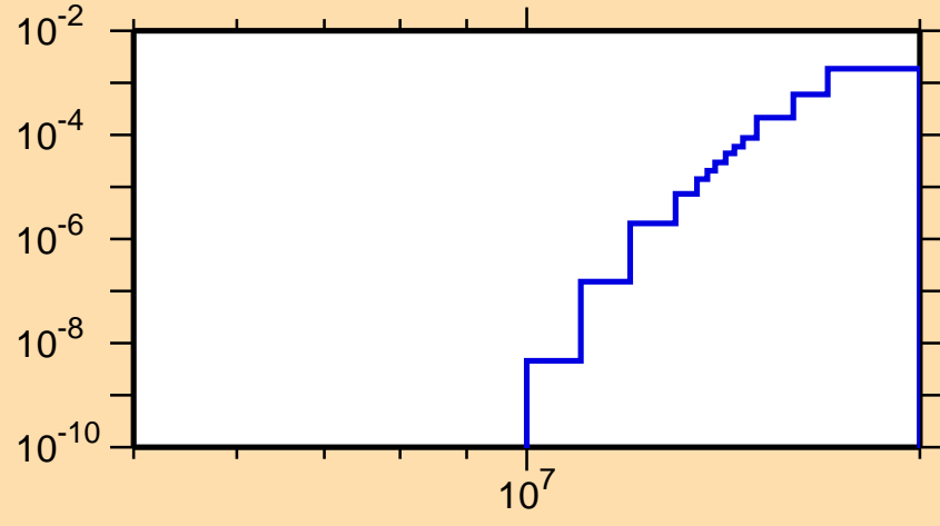
\sigma vs. E for ^{124}\text{La} (mt 45)
