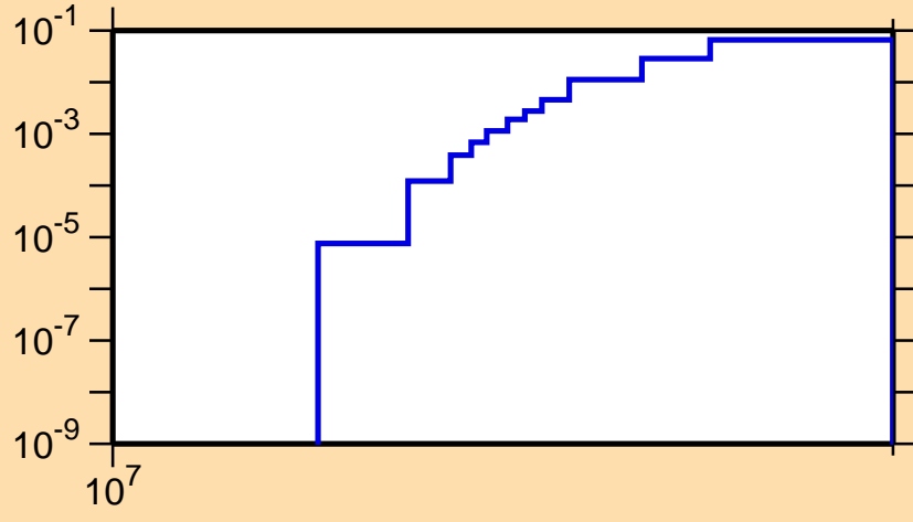
\sigma vs. E for ^{124}\text{La}(n,2np)
