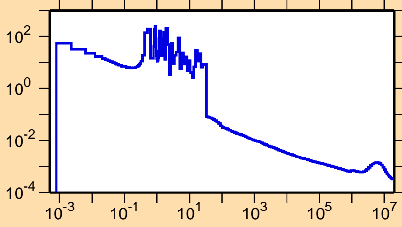
\sigma vs. E for ^{124}\text{La}(n,\gamma)
