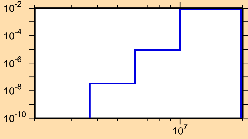
\sigma vs. E for ^{124}\text{La}(n,n\alpha)
