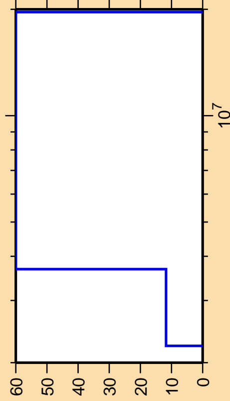
\Delta\sigma/\sigma vs. E for ^{124}\text{La}(n,n\alpha)
