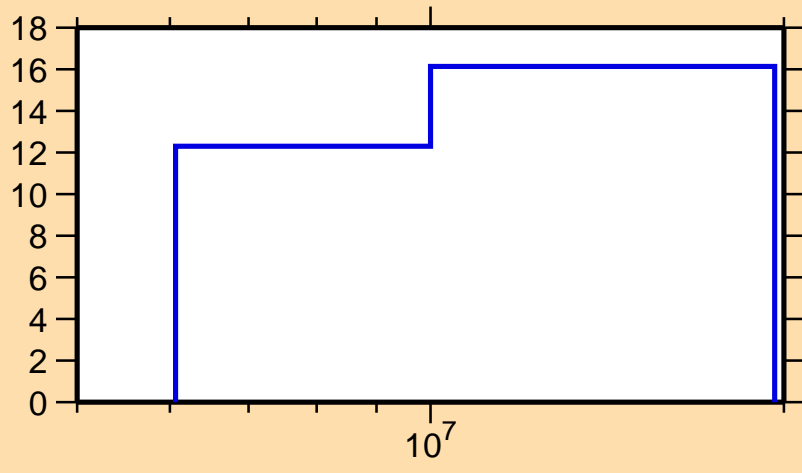
\Delta\sigma/\sigma vs. E for ^{124}\text{La}(n,\text{nonel.})
