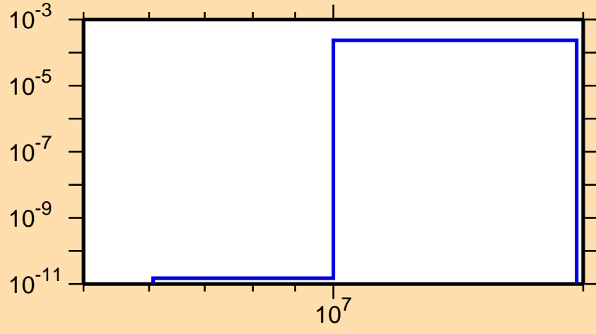
\sigma vs. E for ^{124}\text{La}(n,\text{pd})
