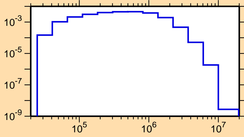
\sigma vs. E for ^{124}\text{La}(n,n_2)
