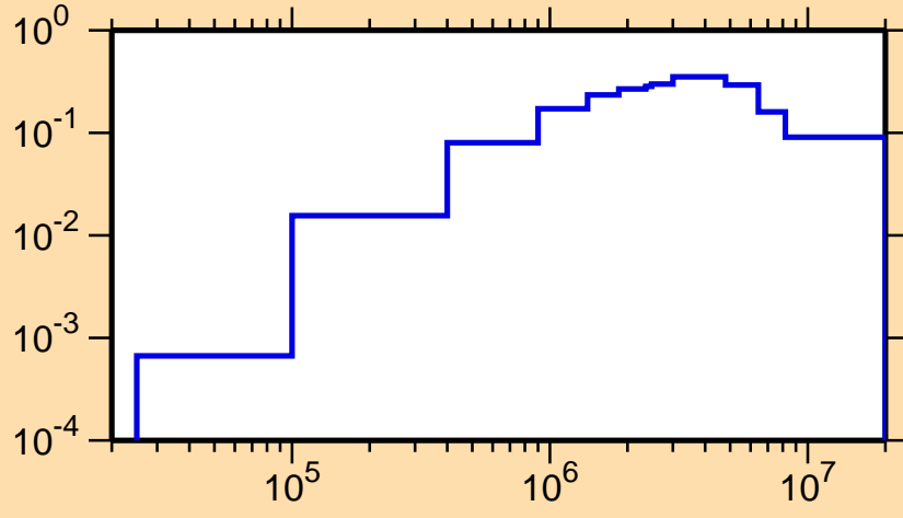
\sigma vs. E for ^{124}\text{La}(n,n\text{cont.})
