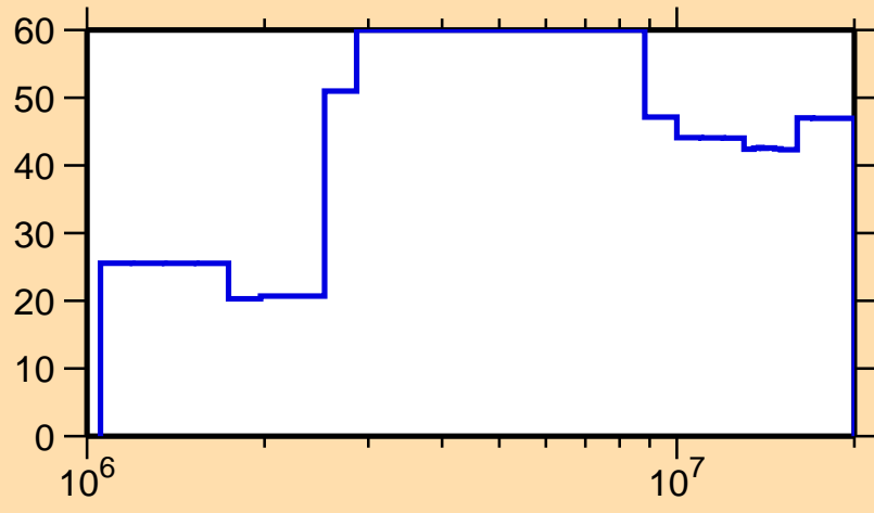
\Delta\sigma/\sigma vs. E for ^{125}\text{La}(n, el.)
