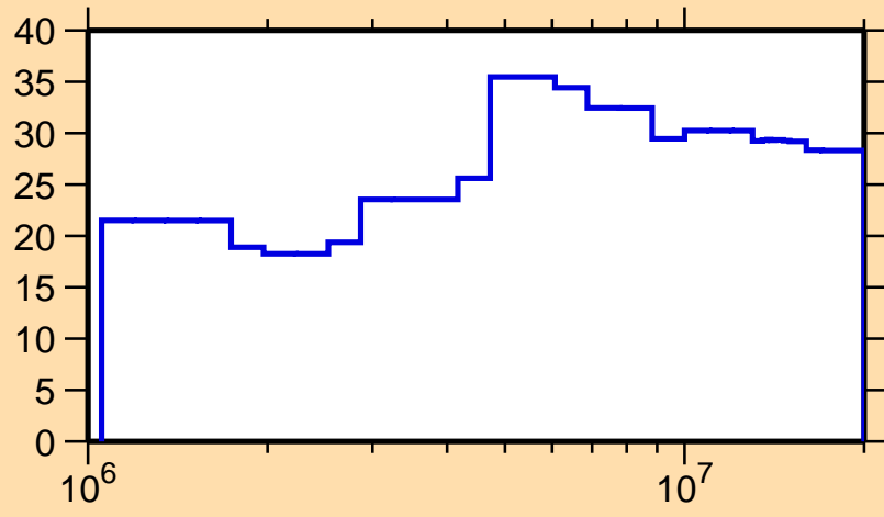
\Delta\sigma/\sigma vs. E for ^{125}\text{La}(n,\text{tot.})
