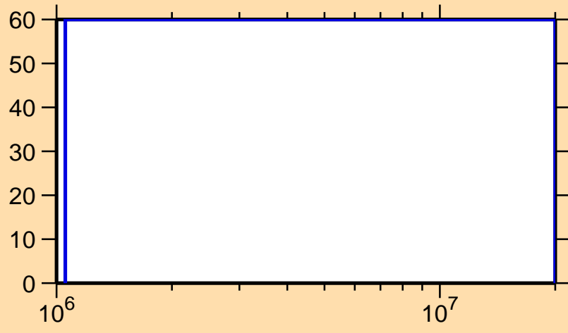
\Delta\sigma/\sigma vs. E for ^{125}\text{La}(n,n_1)
