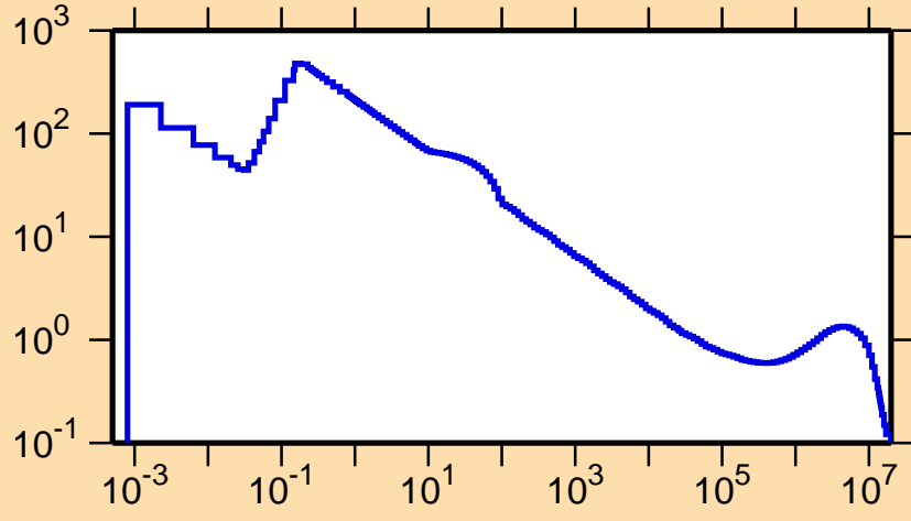
\sigma vs. E for ^{125}\text{La}(n,p)
