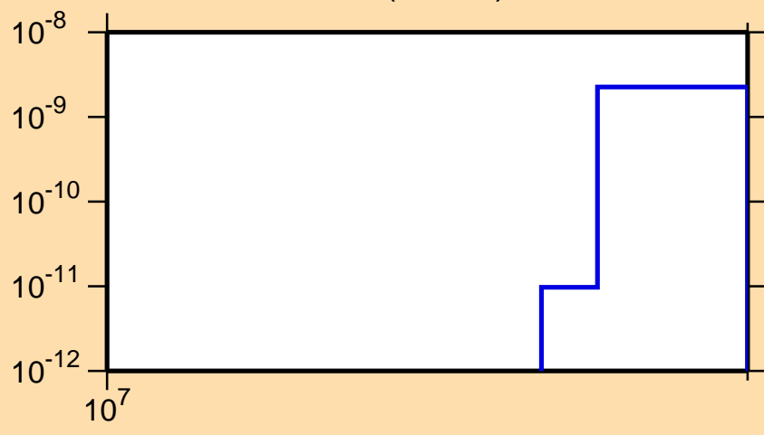
\sigma vs. E for ^{125}\text{La}(n,2n\alpha)
