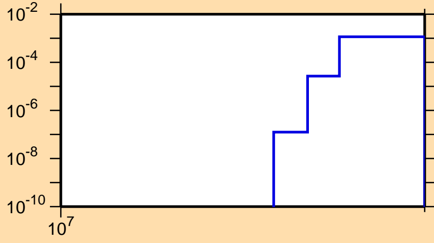
\sigma vs. E for ^{125}\text{La}(n,2np)
