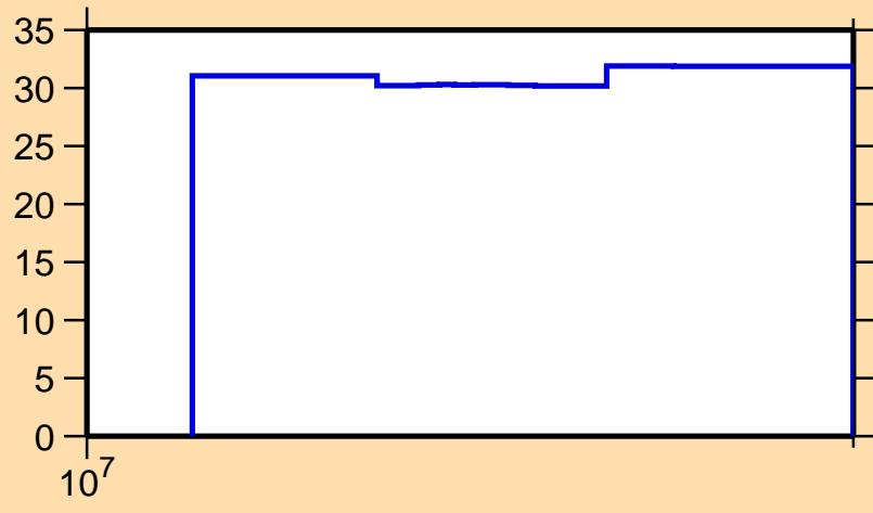
\Delta\sigma/\sigma vs. E for ^{125}\text{La}(n,\text{nonel.})
