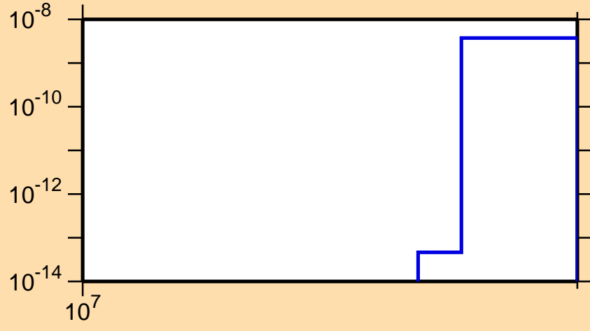
\sigma vs. E for ^{125}\text{La}(n,nt)
