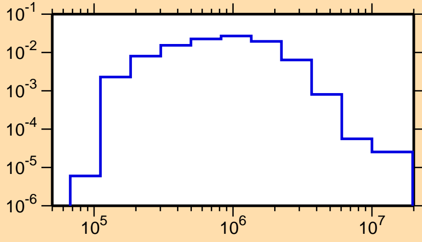
\sigma vs. E for ^{125}\text{La}(n,n_2)
