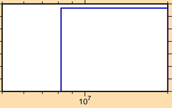
\sigma vs. E for ^{125}\text{La}(n,\text{pt})
